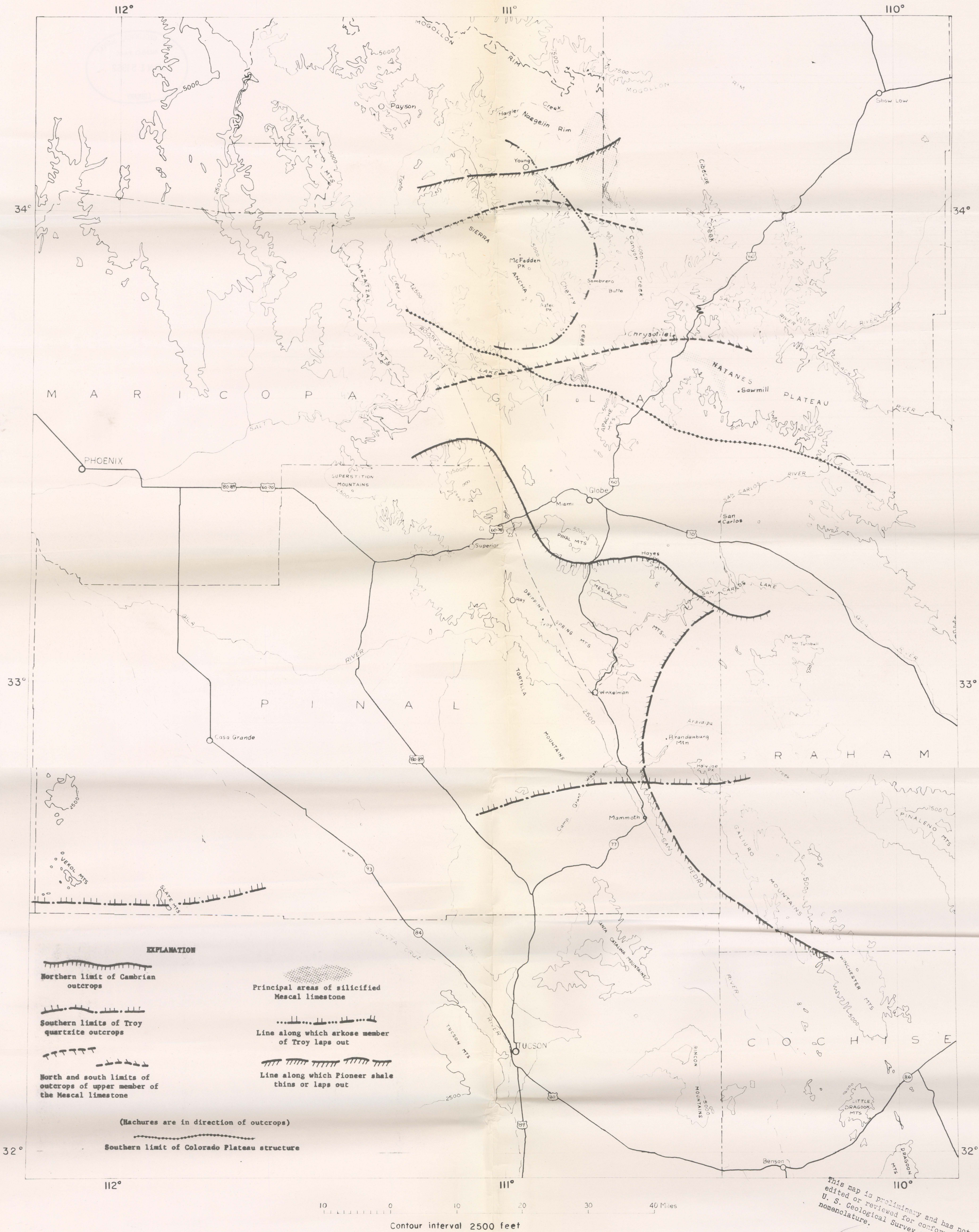
FIGURE 3. INDEX MAP SHOWING POSITIONS OF SOME PALEOGEOGRAPHIC FEATURES OF THE YOUNGER PRECAMBRIAN FORMATIONS
