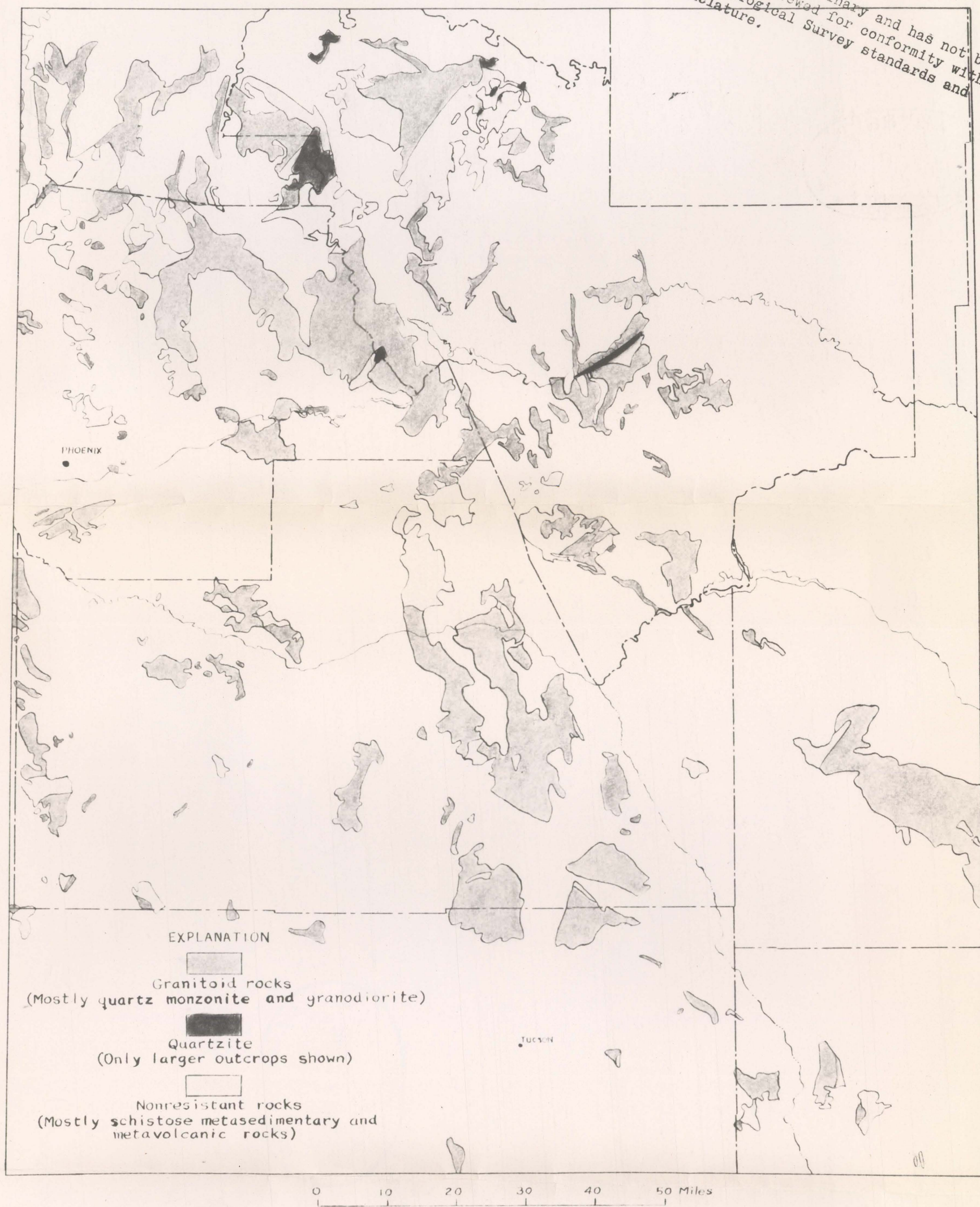
FIGURE 4. SKETCH MAP SHOWING OUTCROPS OF THE OLDER PRECAMBRIAN TERRANE, SUBDIVIDED AS TO ROCK TYPES THAT WOULD CONTRIBUTE DIFFERENT MATERIALS FOR LATE PRECAMBRIAN SEDIMENTATION
