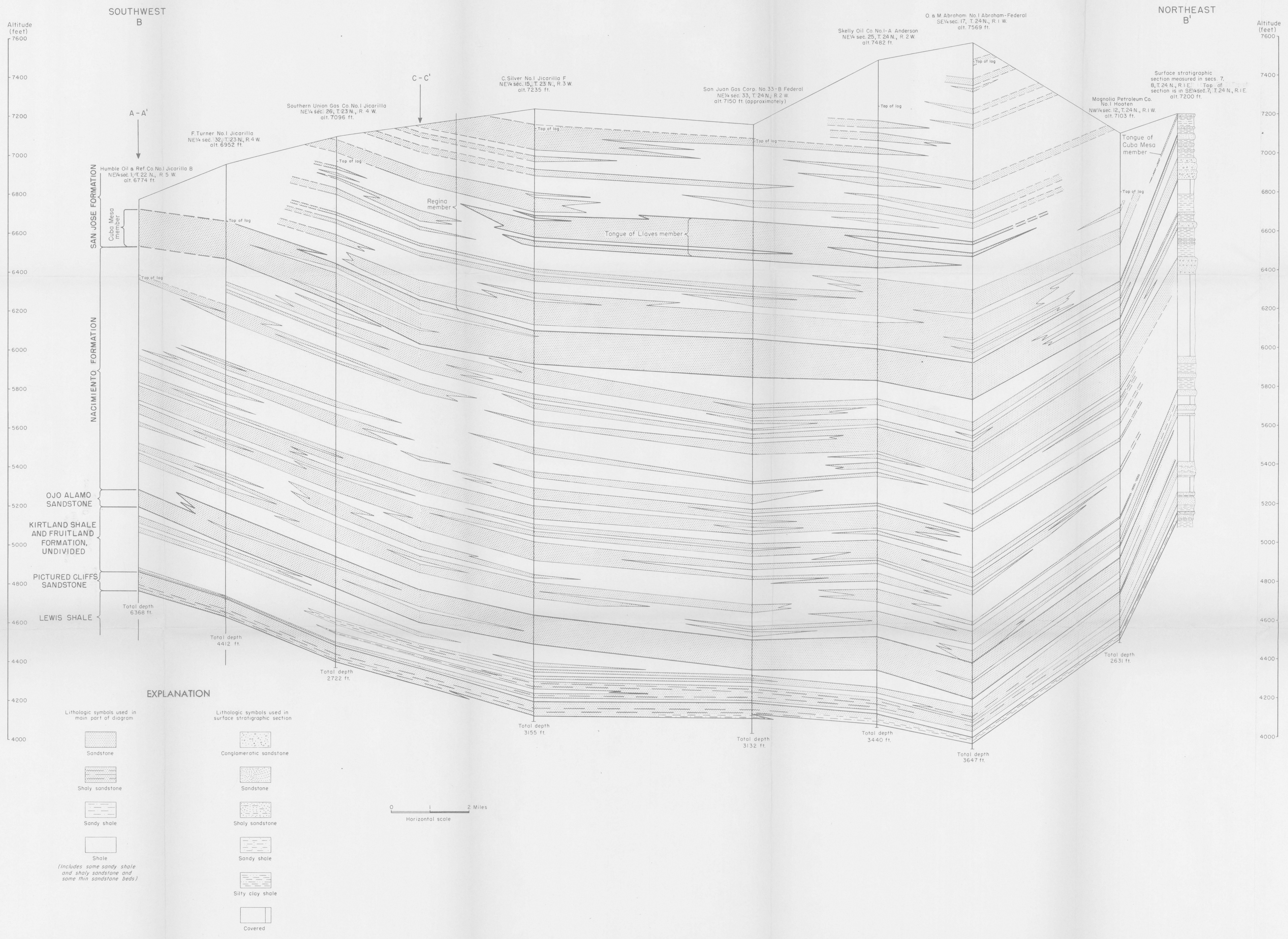
Figure 6.--Diagram showing correlations of rock units as interpreted from electric logs of wells and surface stratigraphic section along line B-B' (shown on Fig. 4).
