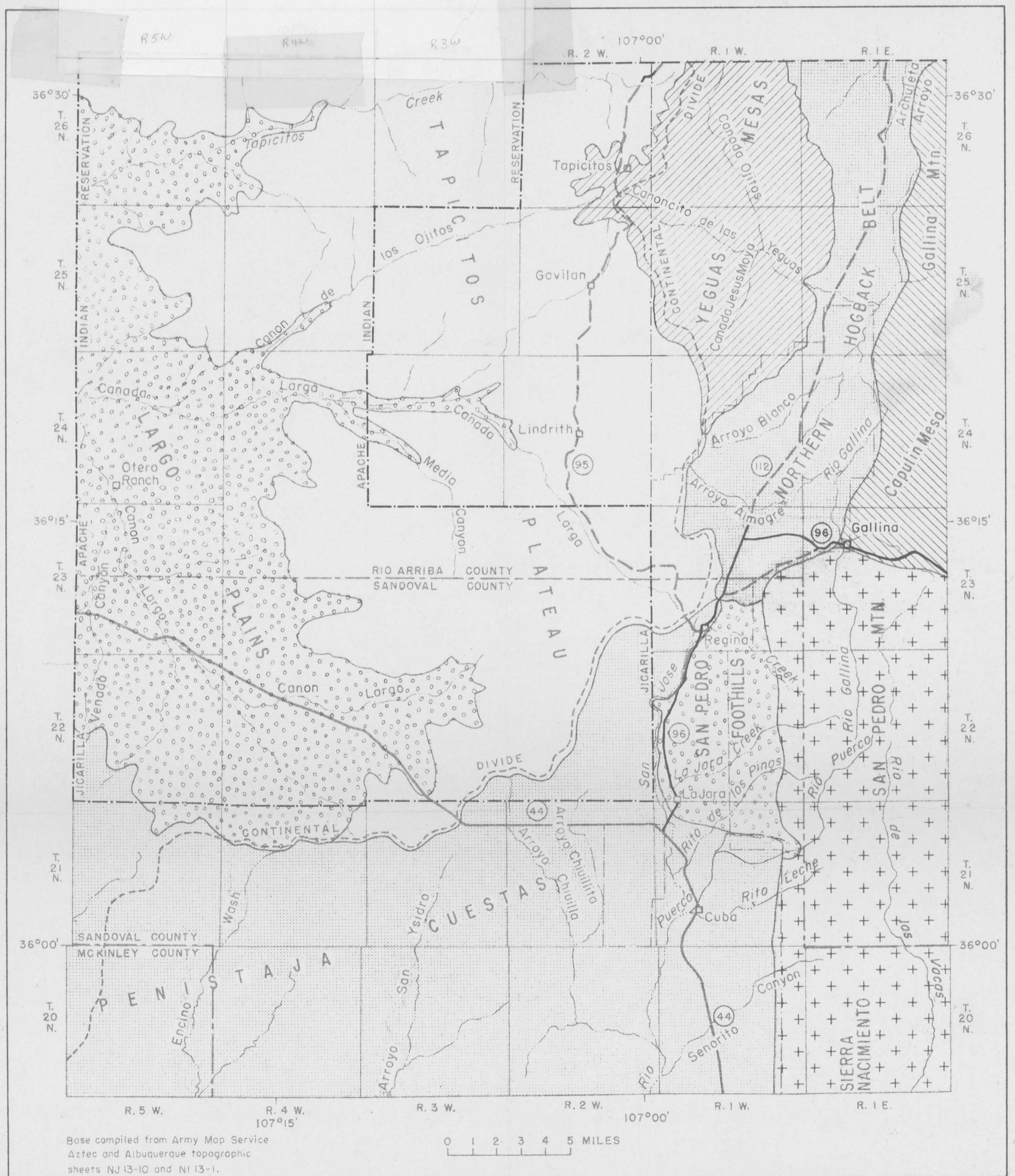
Figure 3.--Physiographic index map of the east-central part of the San Juan Basin and adjacent region, New Mexico
