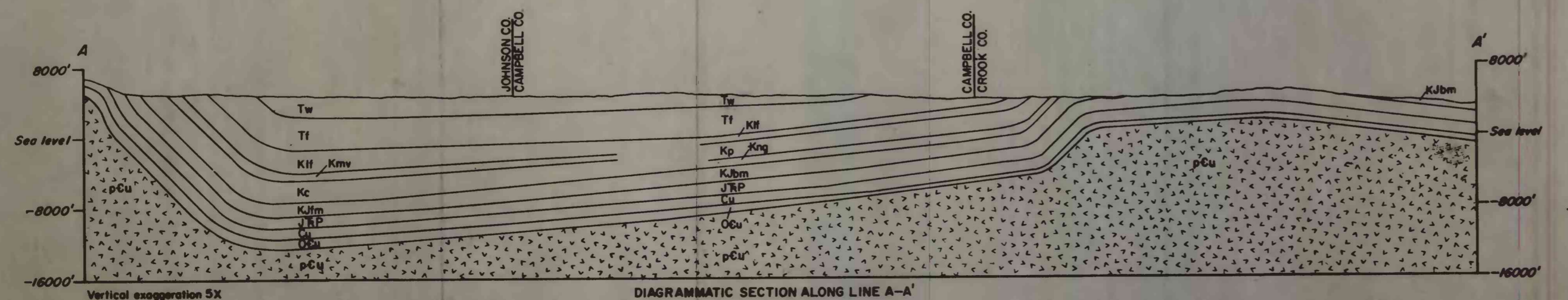
FIGURE 2.--GEOLOGIC MAP AND DIAGRAMMATIC SECTION OF THE POWDER RIVER BASIN, WYOMING AND MONTANA
