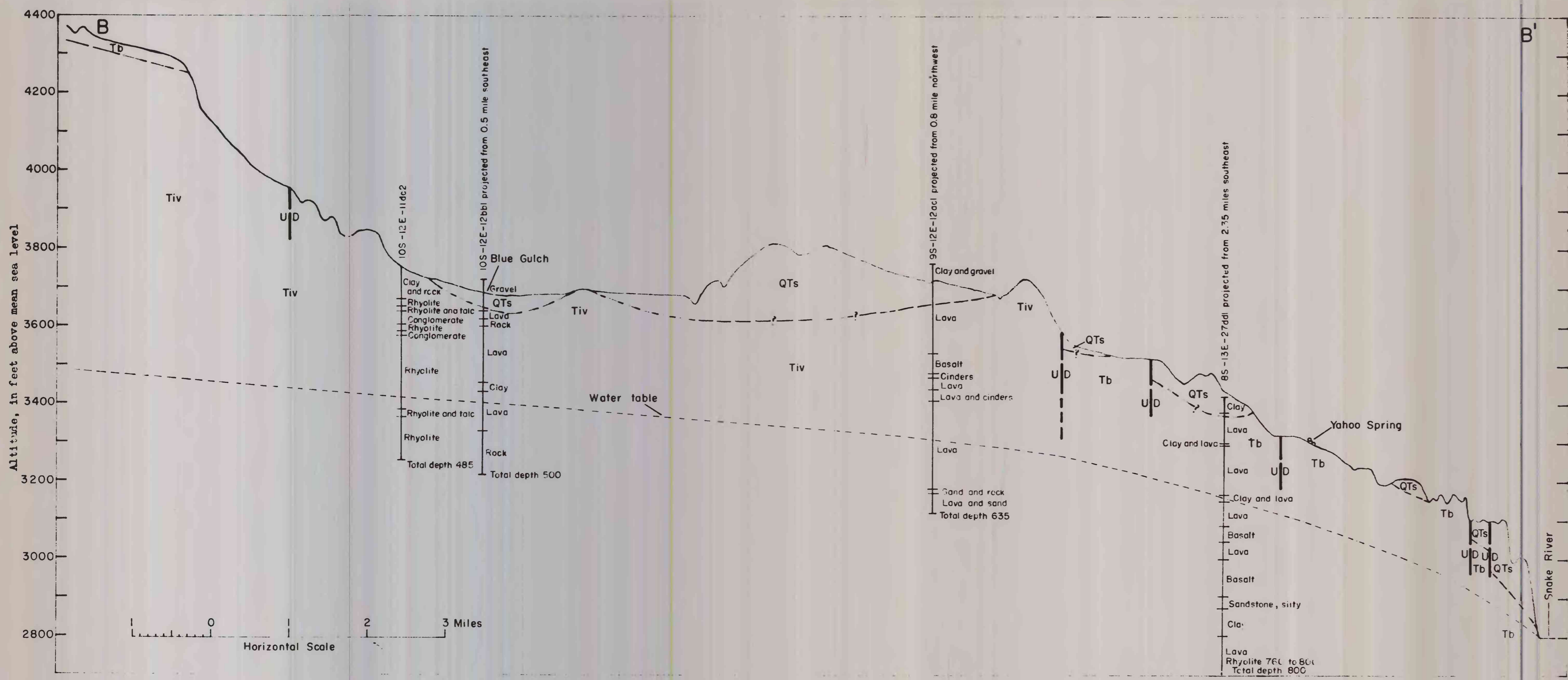
Figure 3.--Geologic section across the eastern part of the Sailor Creek area showing the approximate position of the water table.
