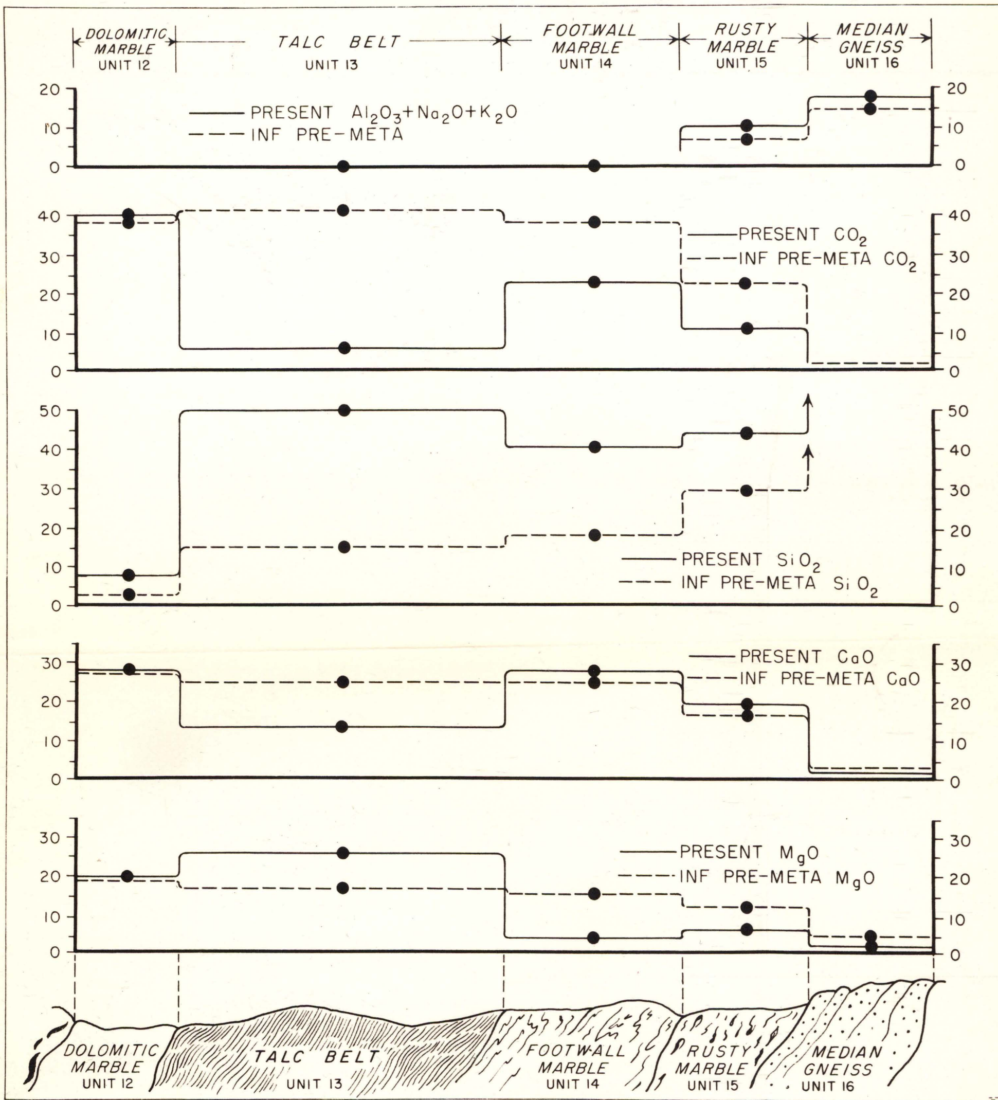
Figure 15. Stratigraphic relations between talc belts and associated lithologic units, and cross-section showing chemical changes believed to have occurred in evolution of those units.
