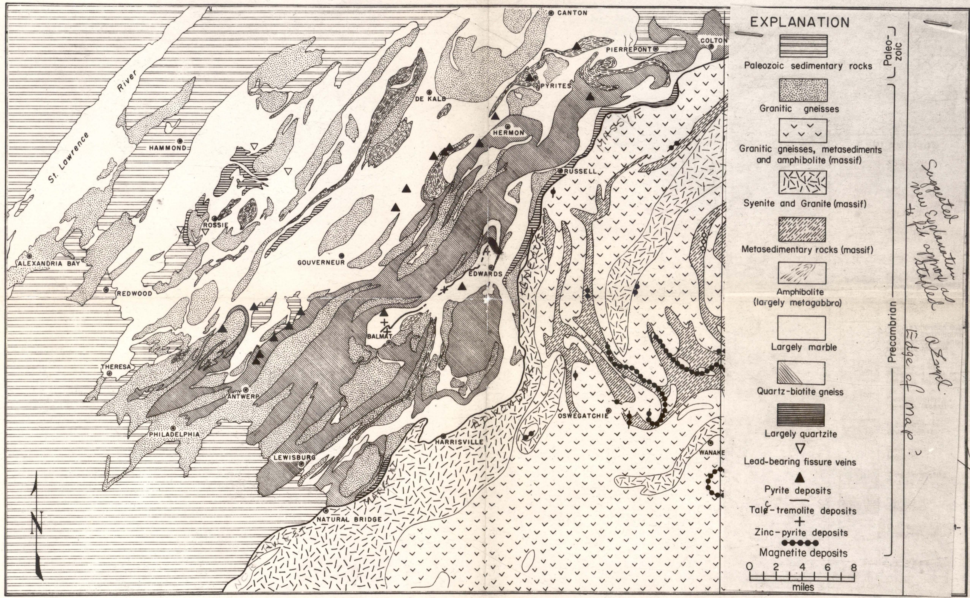
Figure 2. GENERALIZED GEOLOGIC MAP OF THE NORTHWEST ADIRONDACKS SHOWING THE DISTRIBUTION OF MINERAL DEPOSITS From maps compiled by Buddington (1955) and Engel and Engel (1953b). Original work largely by Buddington, Cushing, Leonard, Newland and Smyth.
