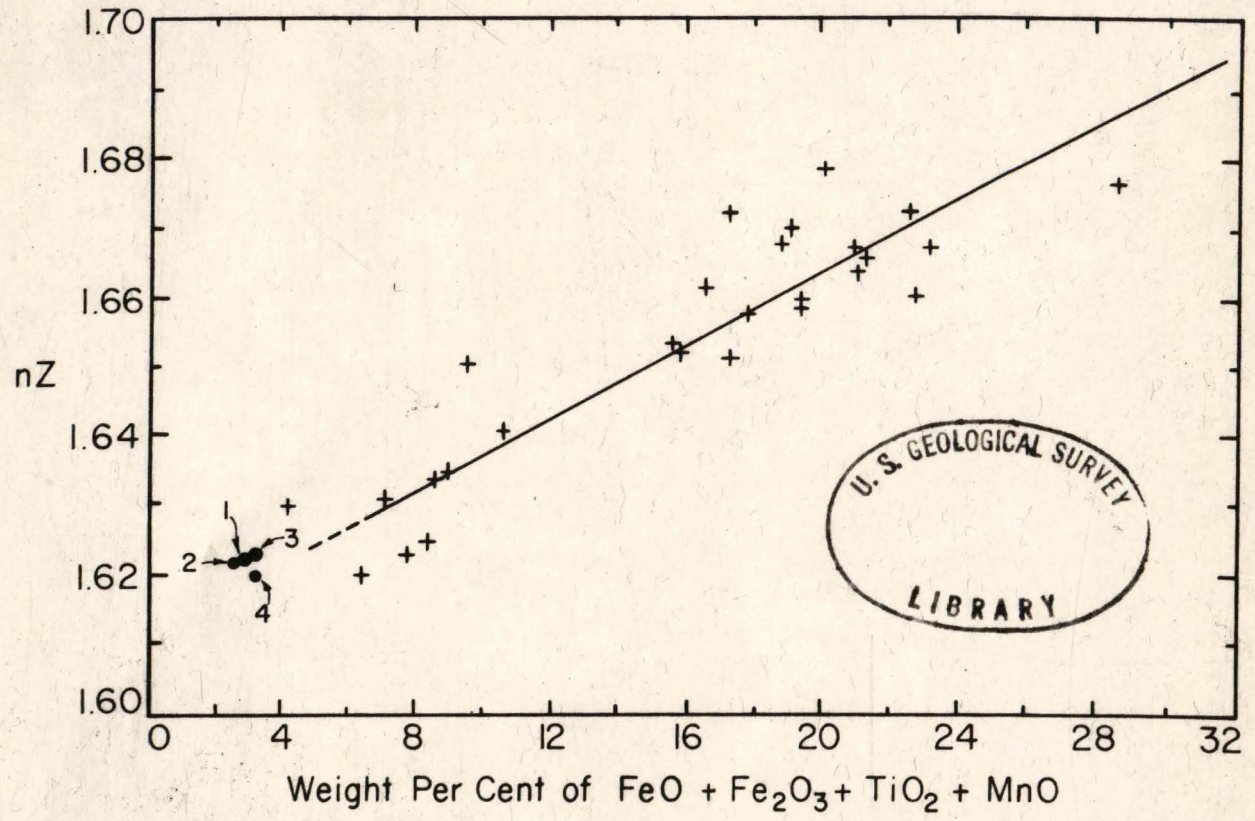
Figure 20. Diagram showing the maximum refractive index in 32 anthophyllites, plotted against weight percent of FeO + Fe 2 O 3 + TiO 2 + MnO. Four of the anthophyllites (dots) are from the talc deposits; and the data for the 28 crosses have been assembled from the literature by Rabbitt (1947), who also constructed the diagram.
