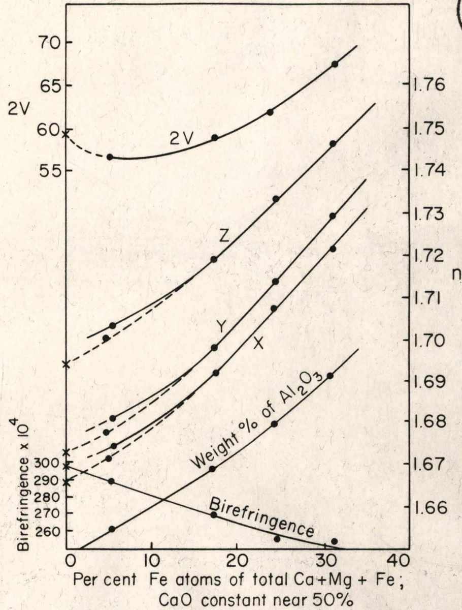
Figure 21. Optical properties of diopsides from the Balmat-Edwards district (crosses) compared with those of other diopsides as recorded by Hess (1949).
