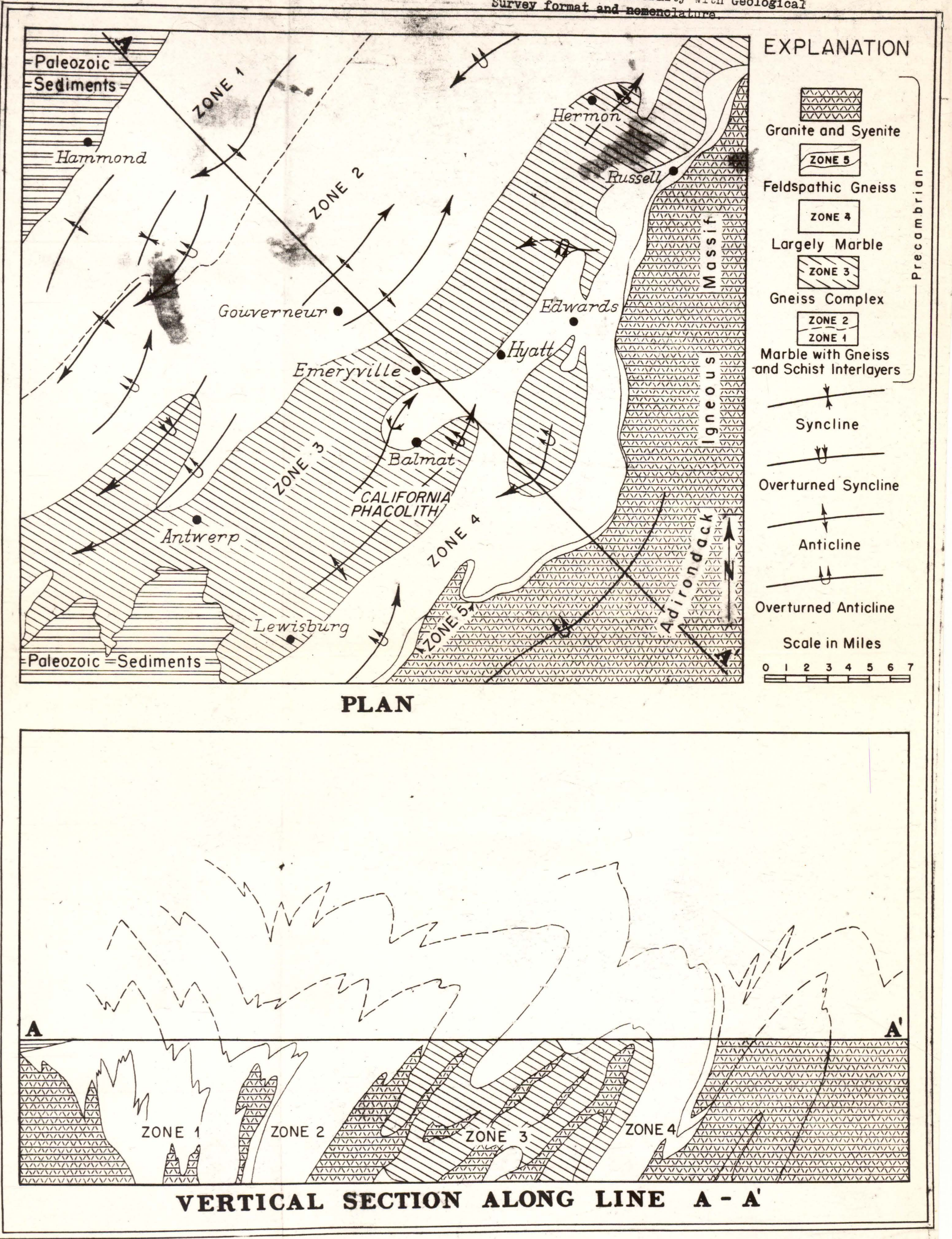
Figure 3: Generalized plan and section showing the major structural features in the Grenville series of the northwestern Adirondacks, New York.
