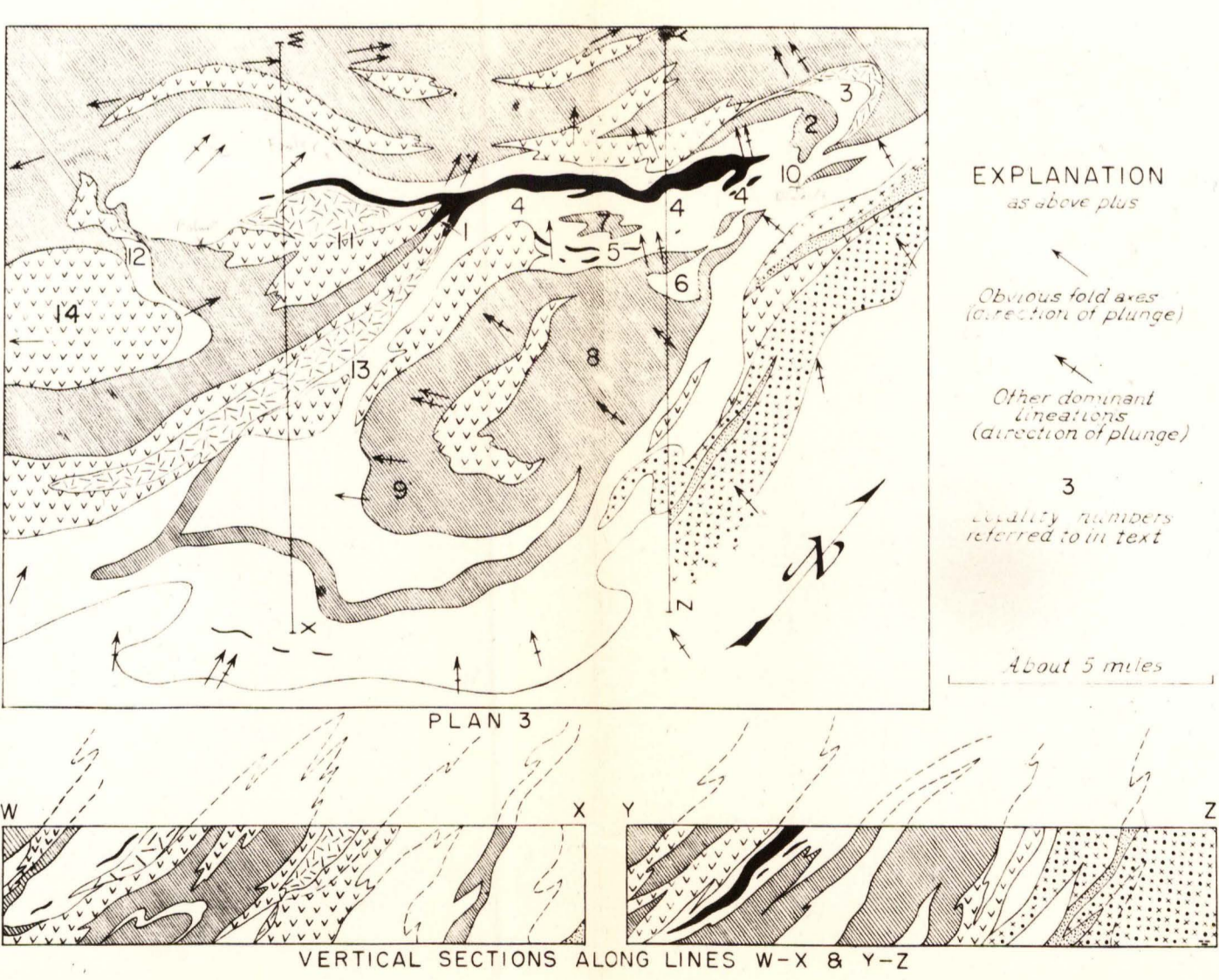
Figure 7. Diagrammatic sketches illustrating the inferred development of structural features in the Balmat-Edwards district.
