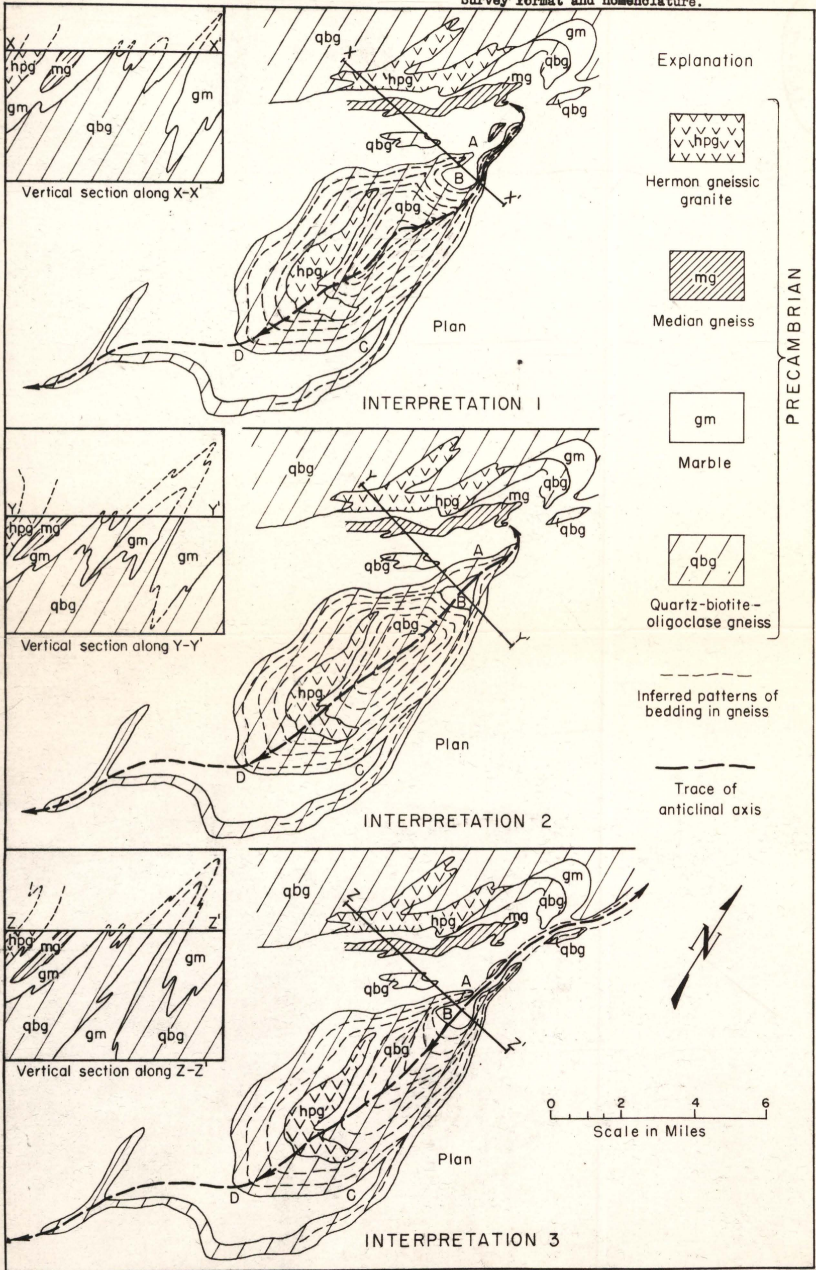
Figure 9. Diagrammatic sketches of the form of the elliptical body of garnetiferous quartz-biotite gneiss south of Edwards, New York (South Edwards gneiss), showing three possible interpretations of its structural form.
