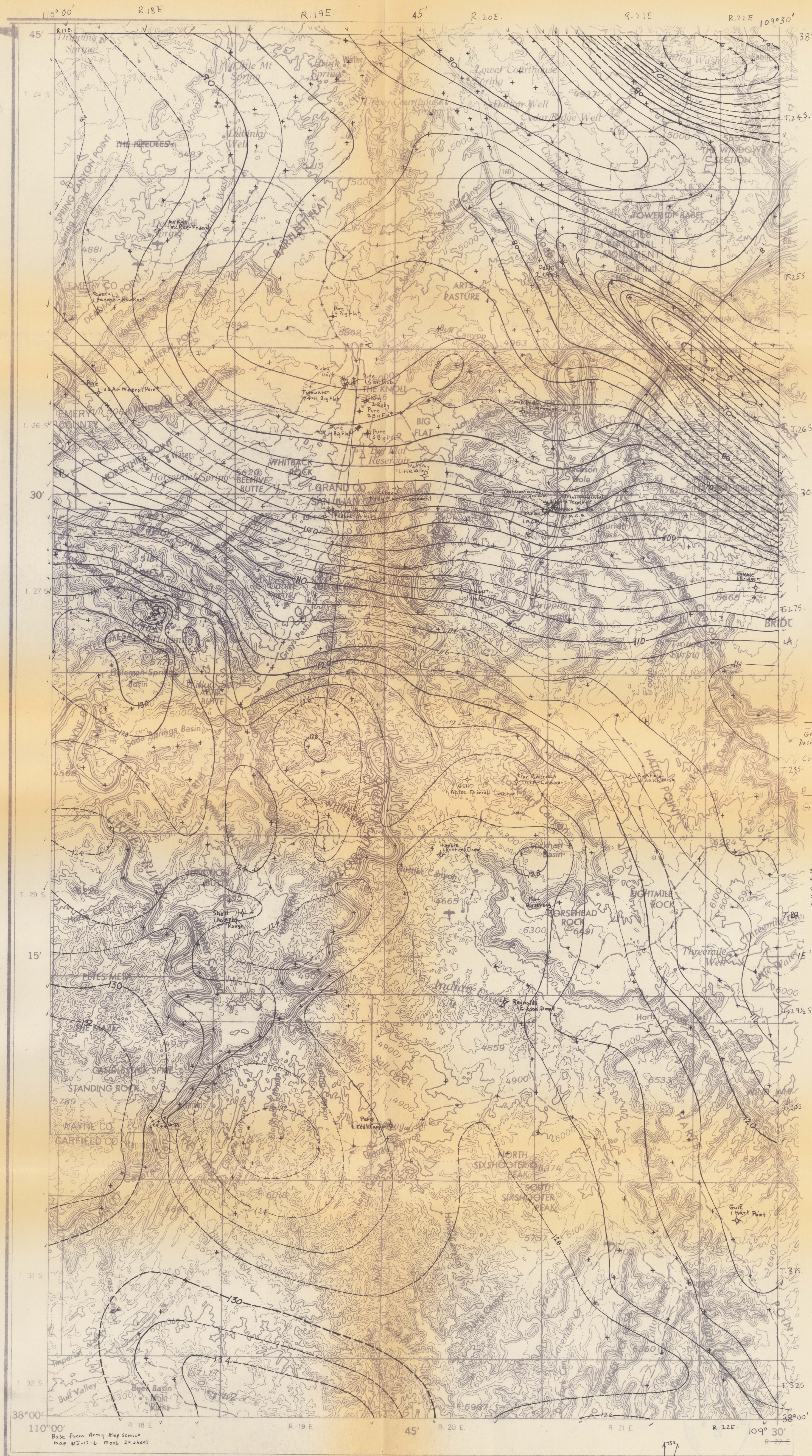
GRAVITY ANOMALY MAP OF THE MOAB-NEEDLES AREA, UTAH
