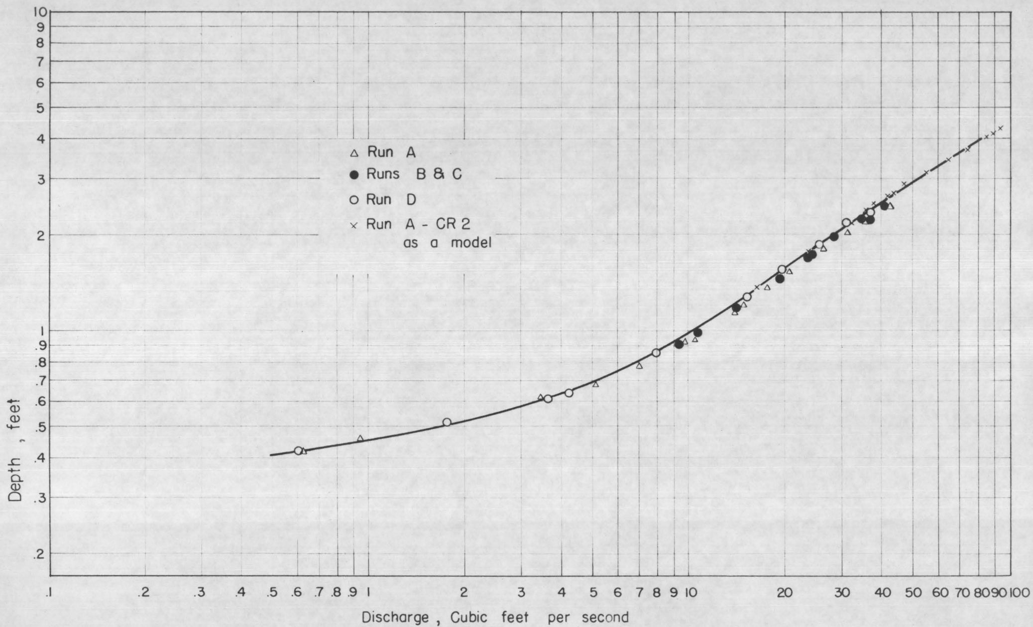
Figure 13. Depth-Discharge relation for Gibecue Ridge No. 1 Control.
