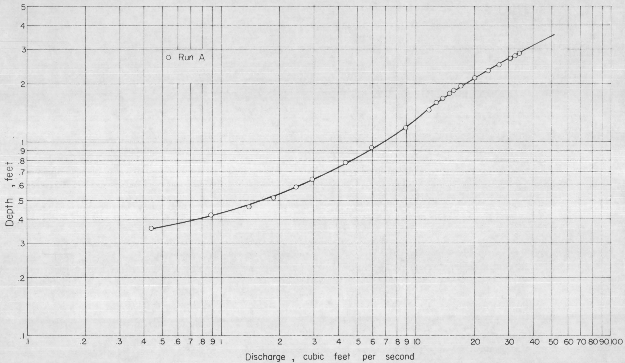
Figure 15. Depth - Discharge Relation for Cibecue Ridge No. 2 Control.
