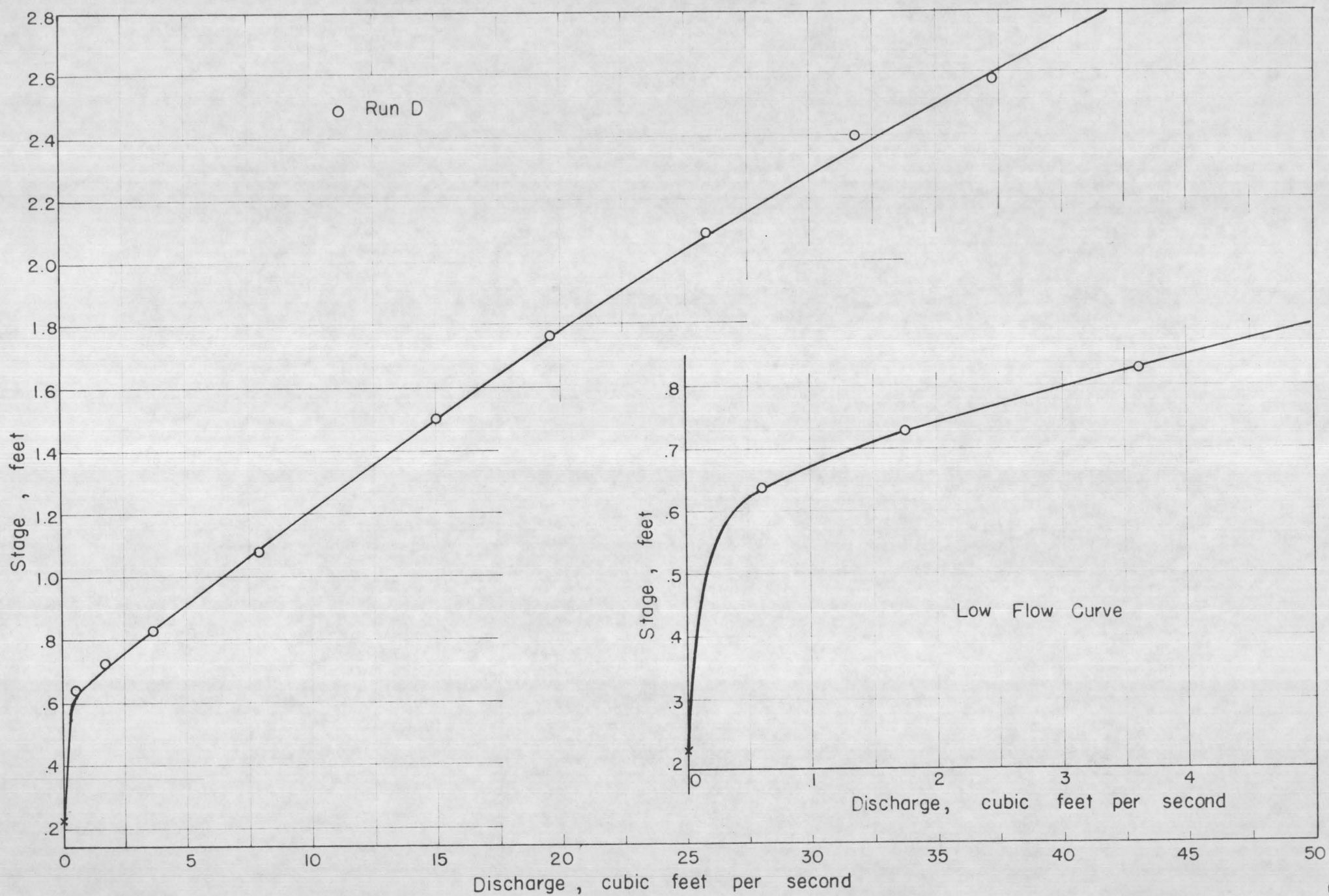
Figure 14. Stage - discharge Relation for Cibecue Ridge No. 1 Control.
