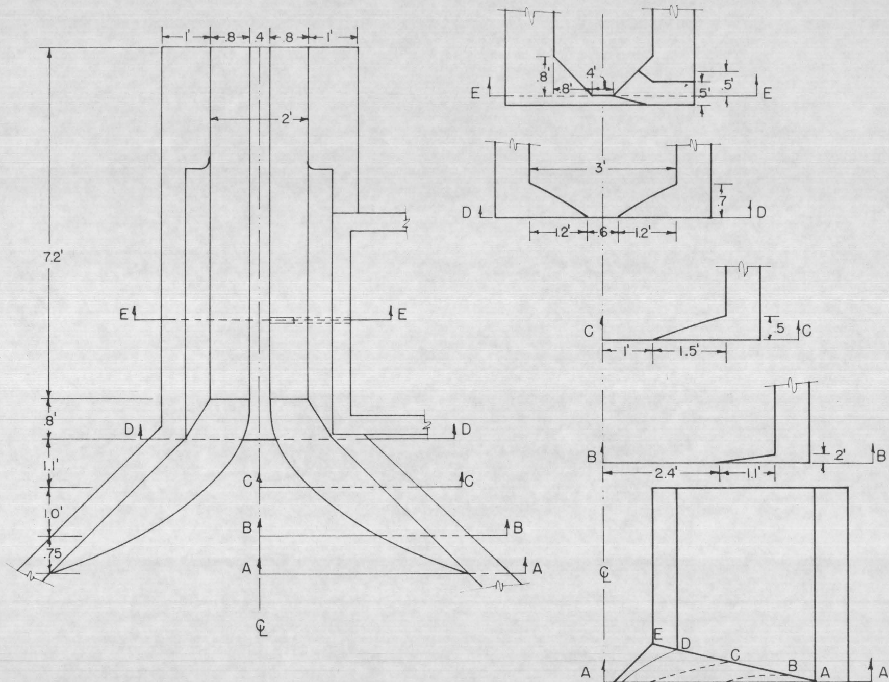
Figure 21. Plan and Cross Section of Modified Cibecue Ridge No. 2 Control. (Scale: 1"=2')
