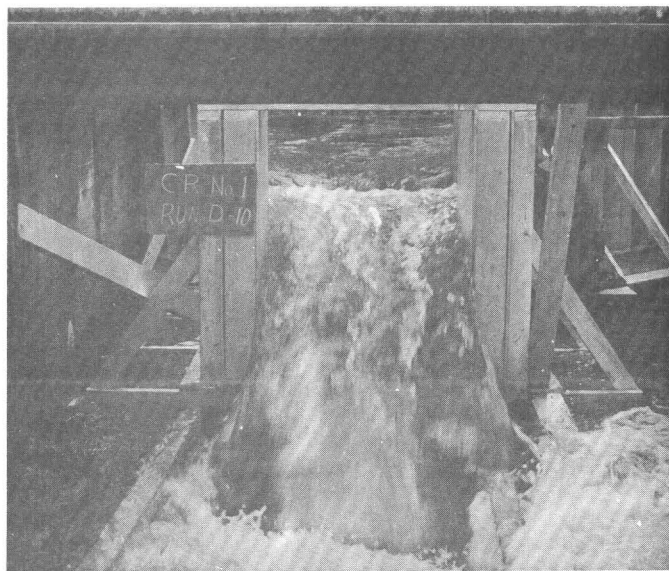
D. Upstream view of Run D-10 Discharge 37.3 cfs
