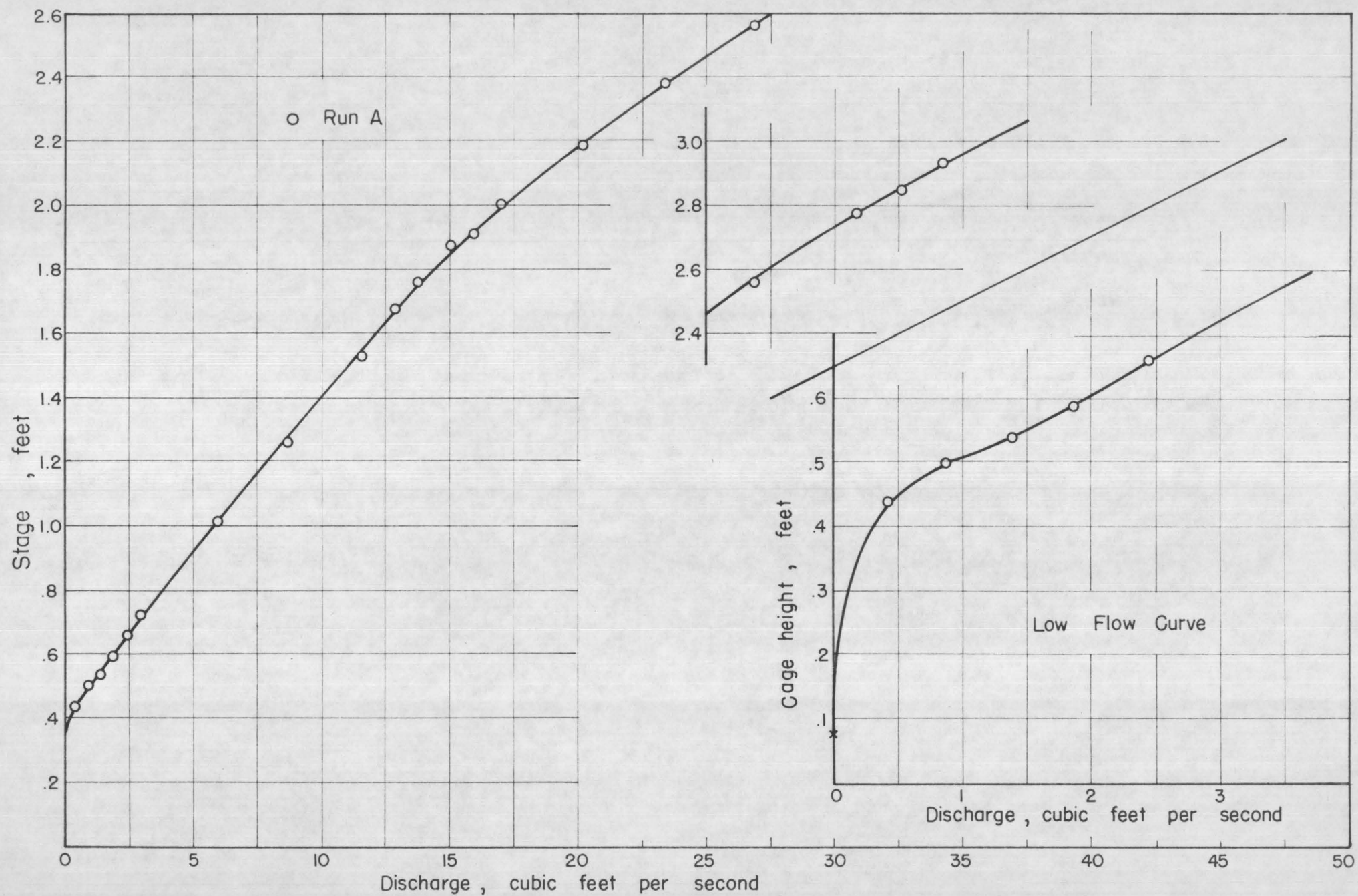
Figure 16. Stage-Discharge Relation for Gibecue Ridge No. 2 Control.
