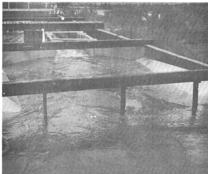
C. Downstream view of Run D-10 Discharge 37.3 cfs
