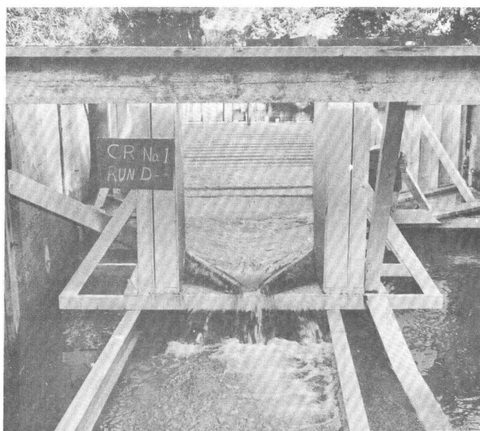
B. Upstream view of Run D-3 Discharge 0.60 cfs
