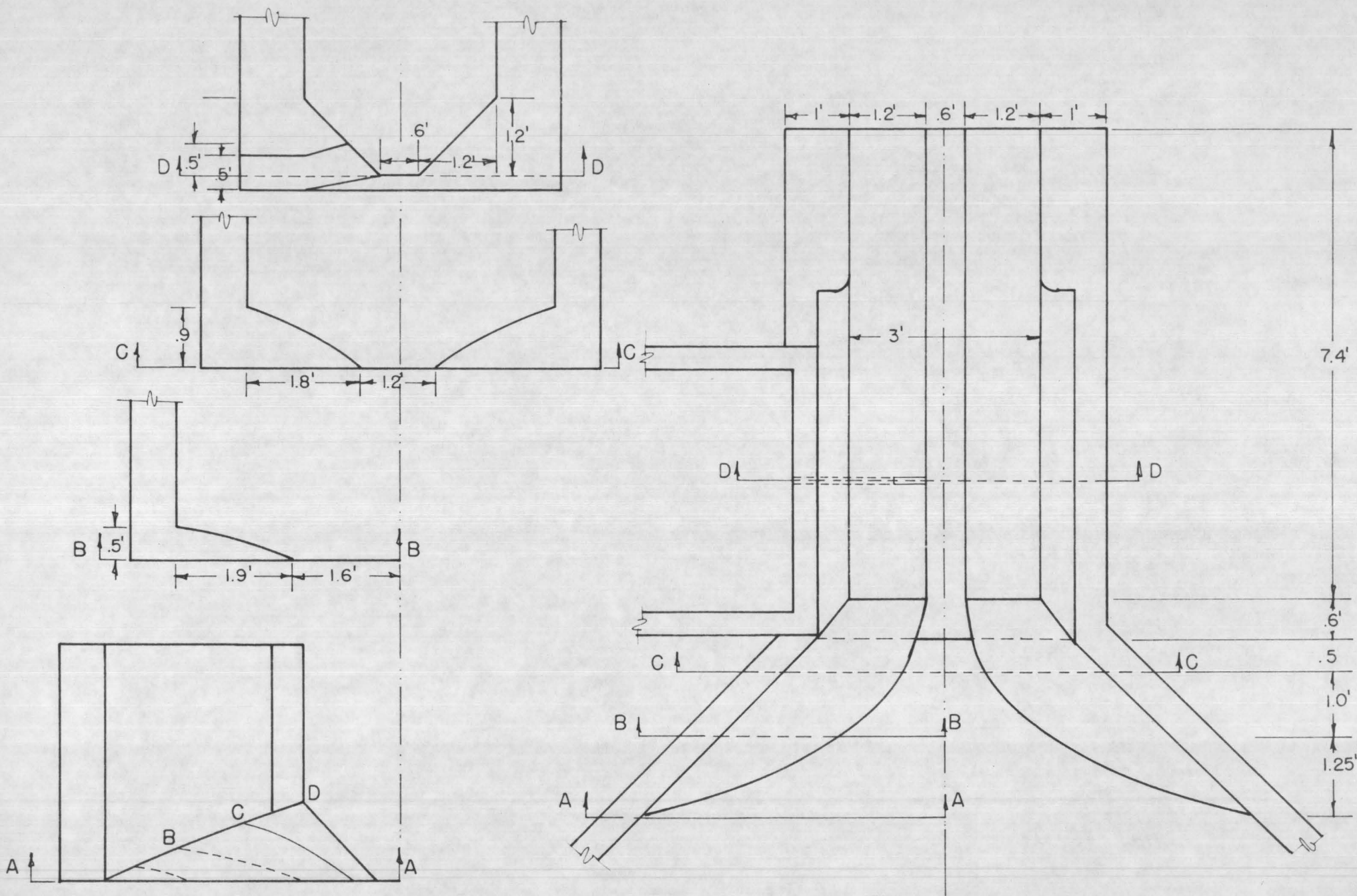
Figure 19. Plan and Cross Section of Modified Cibecue Ridge No. 1 Control. (Scale: 1"=2')
