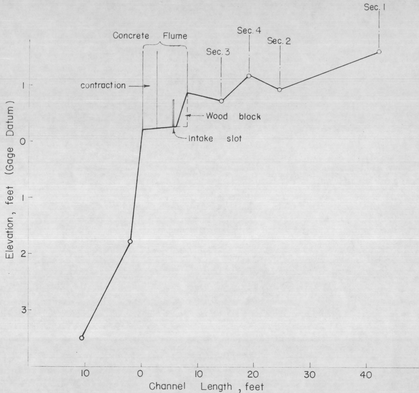
Figure 4. Profile of the control structure and stream bed for Cibecue Ridge No. 1
