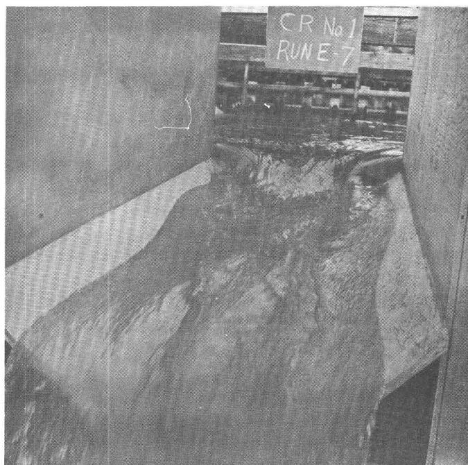
D. Upstream view of Run E-7 Discharge 9.38 cfs
