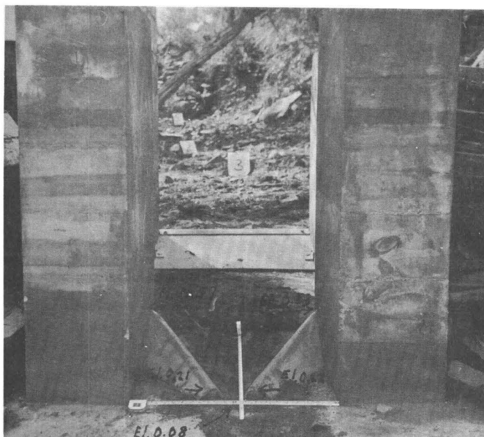
A. Upstream view showing low-water constriction
