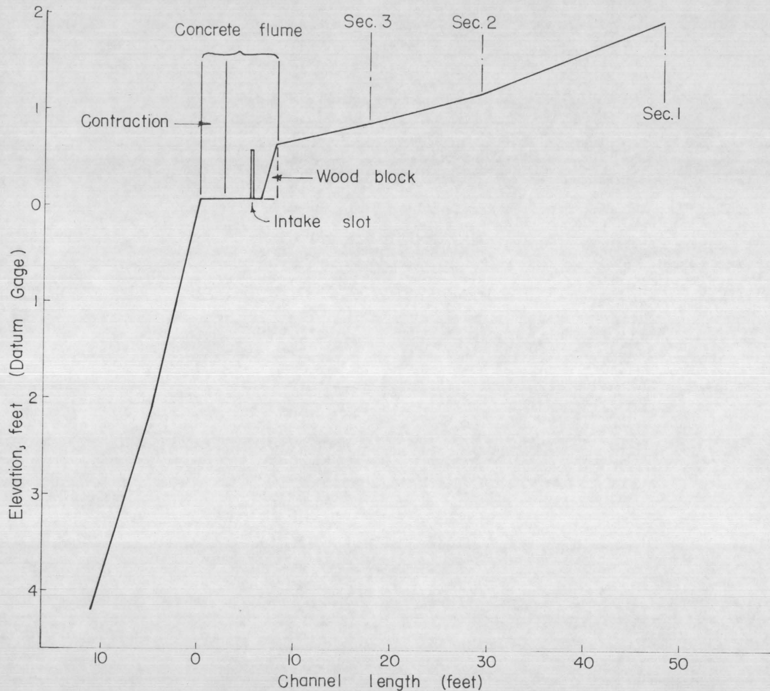
Figure 10. Profile of the control structure and stream bed for Gibecue Ridge No. 2
