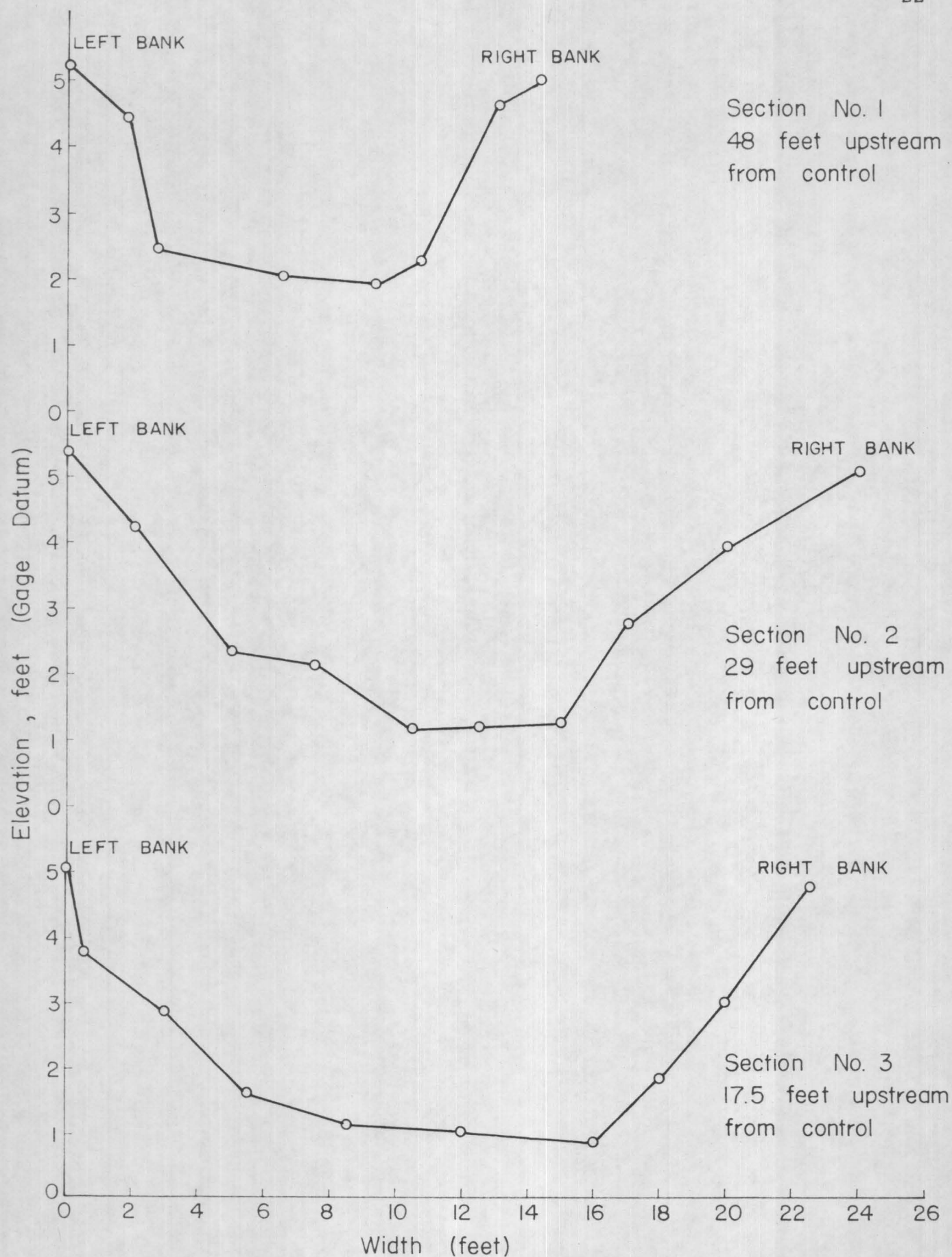
Figure // . Cross-Sections of the approach channel for Cibecue Ridge No. 2
