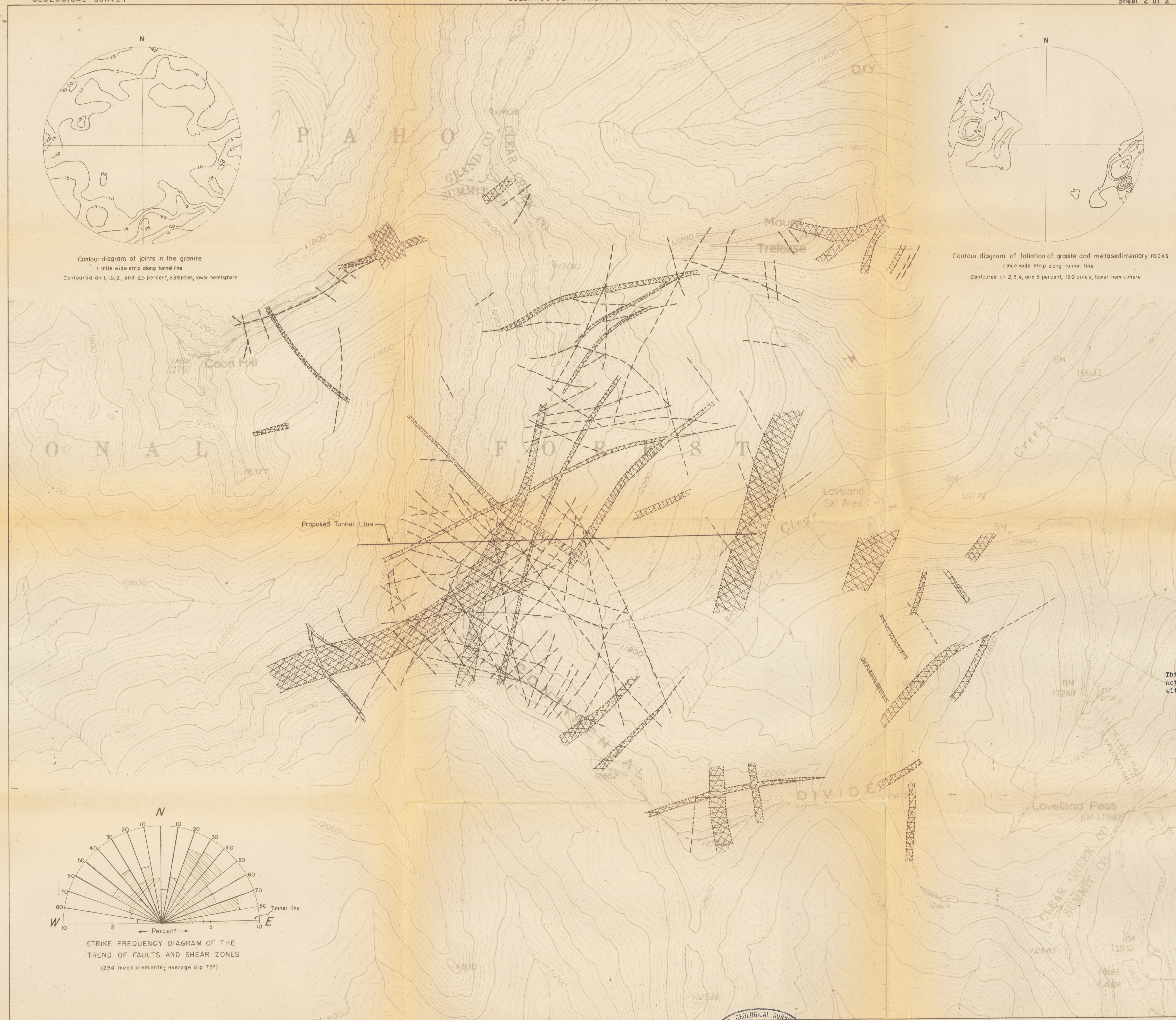
Figure 2B GEOLOGIC MAP OF THE STRAIGHT CREEK TUNNEL AREA: FAULTS AND SHEAR ZONES
