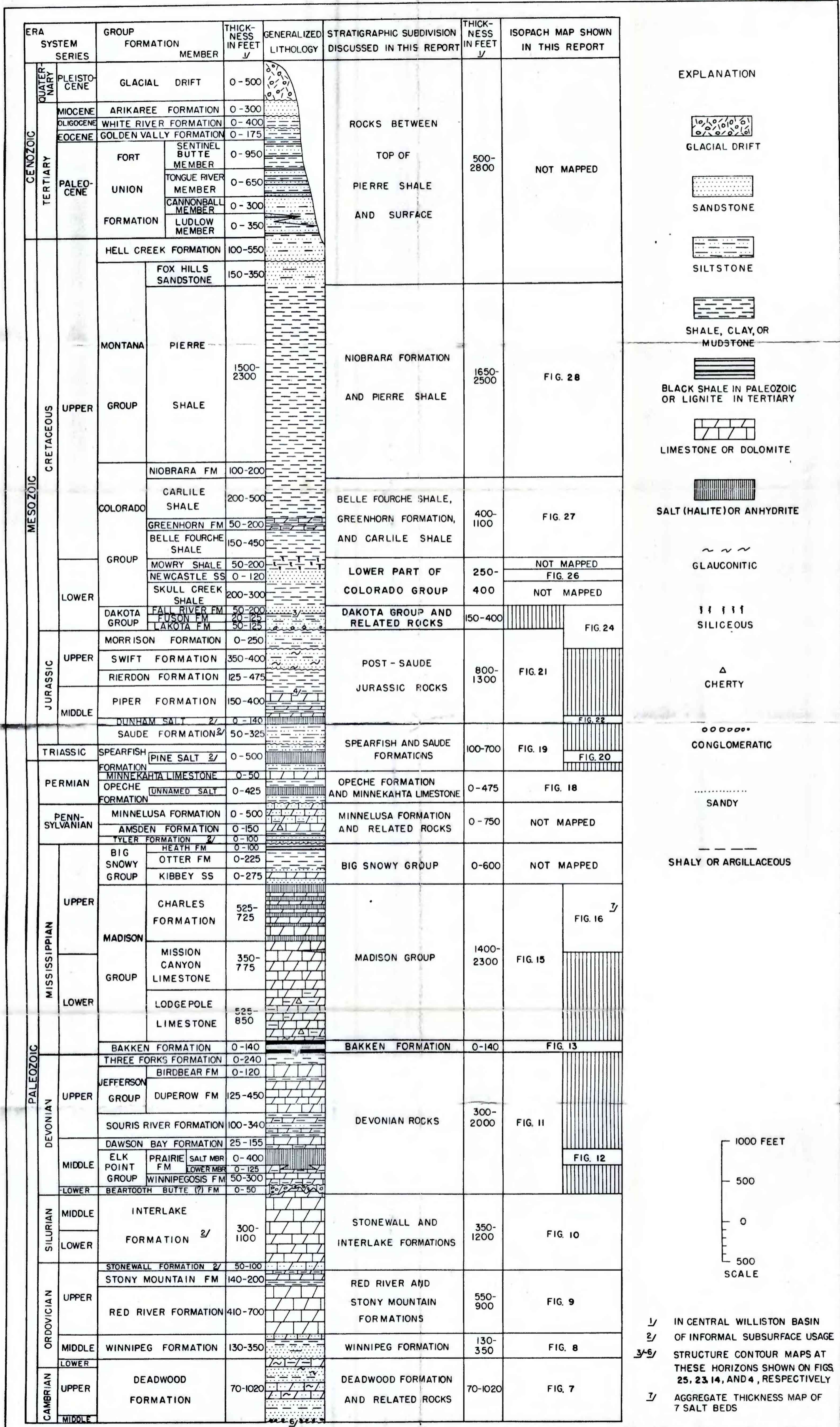
FIGURE 5. GENERALIZED STRATIGRAPHIC SECTION OF SEDIMENTARY ROCKS IN CENTRAL WILLISTON BASIN
