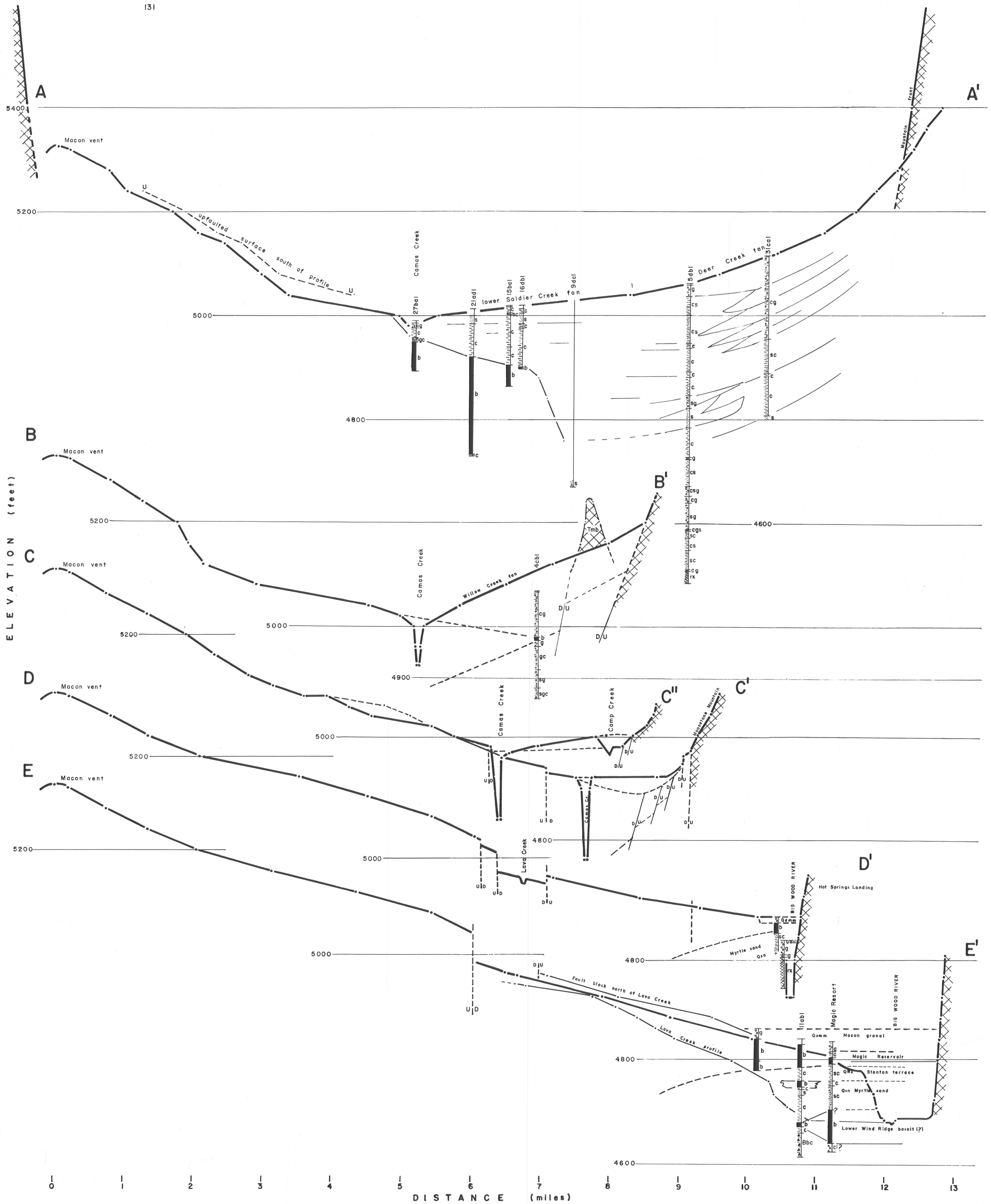
FIGURE 35. --Profile-sections across the Macon basalt flow in eastern Camas Valley. Sections AA' and BB' are across the principal lava dam where Camas Creek was blocked. Section DD' is across the lava dam where Rock Creek was blocked. Vertical exaggeration is about 1:40. Symbols are the same as on the geologic map (pl. 1). Profile lines are located in figure 40 (appendix).
