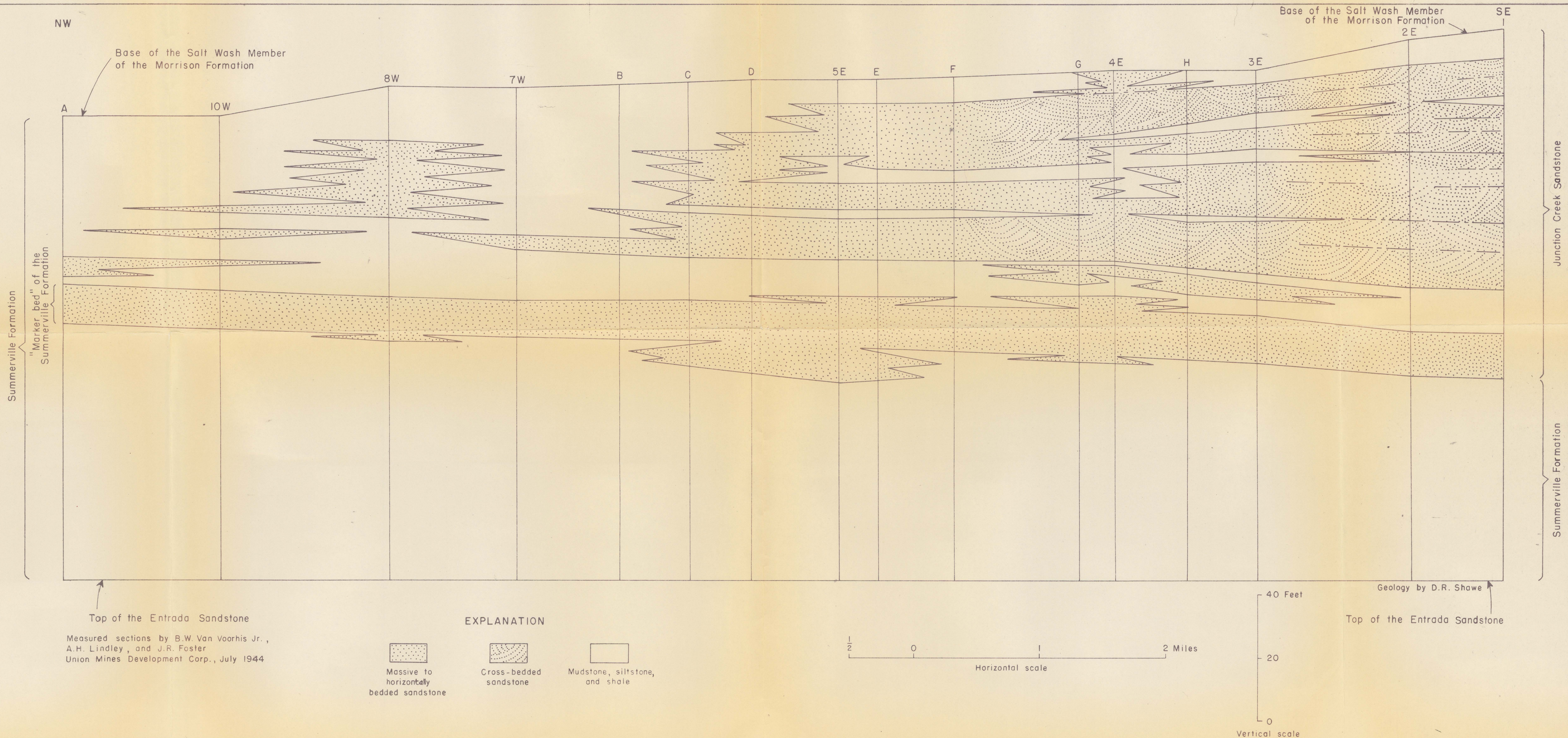
FIGURE 3.-VERTICAL DIAGRAM SHOWING PROBABLE CORRELATIONS OF MEASURED SECTIONS AND RIM SKETCHES OF PARTS OF THE SUMMERVILLE FORMATION AND JUNCTION CREEK SANDSTONE, DOLORES COUNTY, COLORADO
