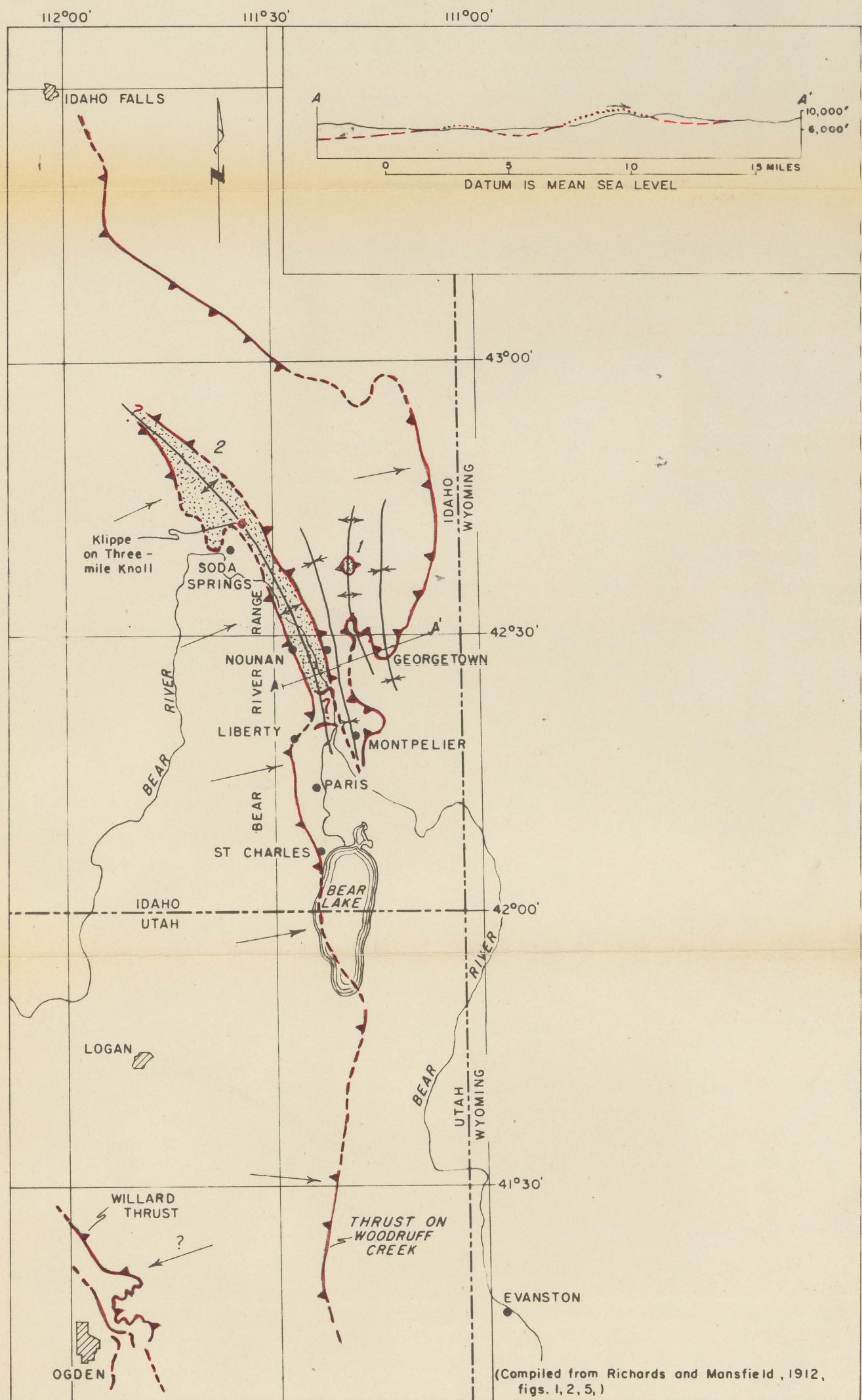
B. THE BANNOCK OVERTHRUST AS ORIGINALLY INTERPRETED BY RICHARDS AND MANSFIELD
