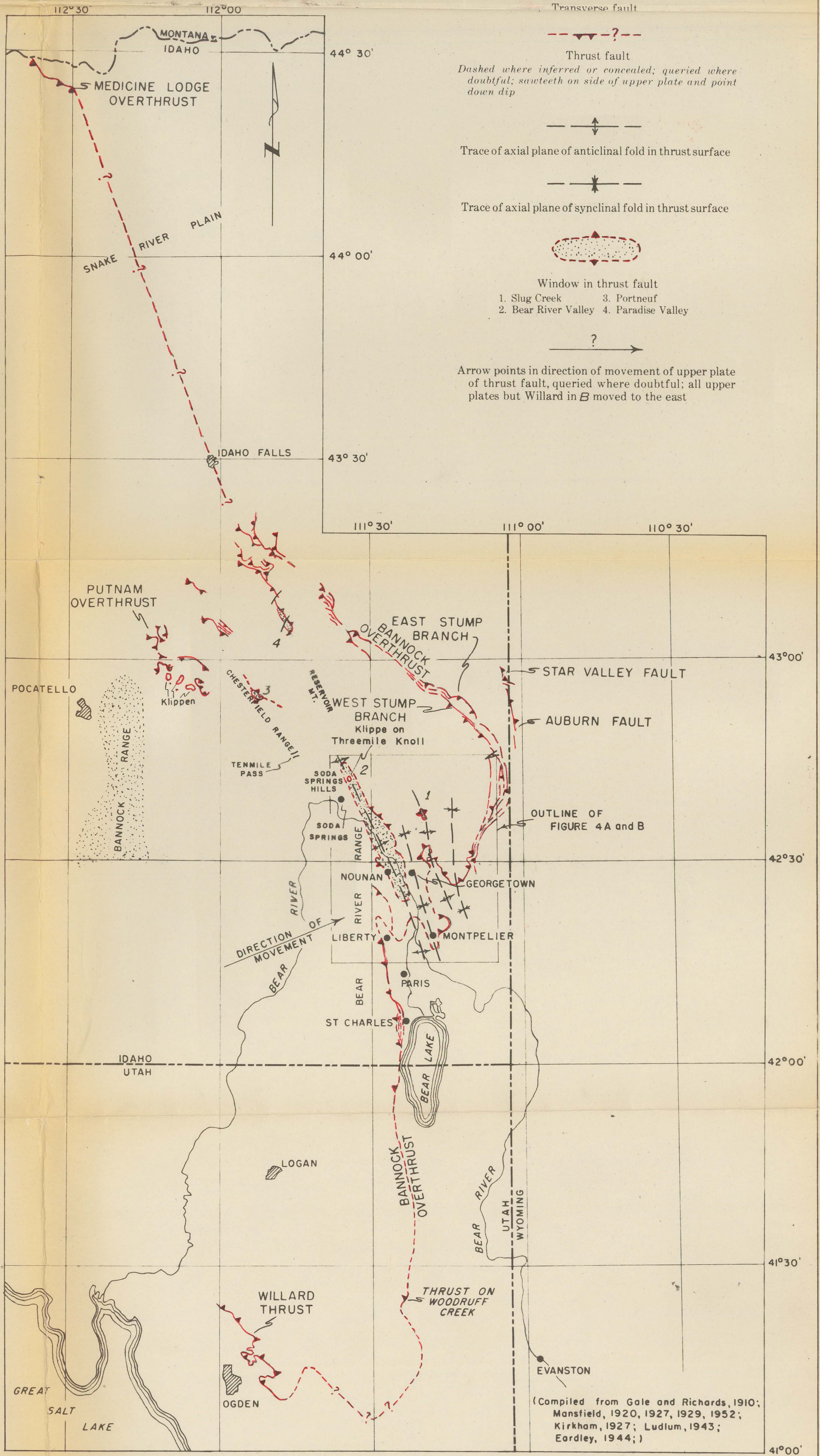
C. MANSFIELD'S FINAL INTERPRETATION OF THE BANNOCK OVERTHRUST, AND CORRELATIONS OF THE BANNOCK WITH OTHER FAULTS AS SUGGESTED BY MANSFIELD AND OTHERS
