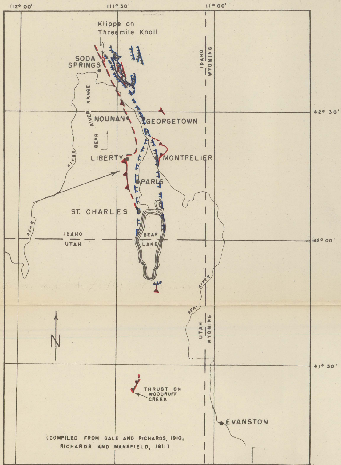
A. STRUCTURAL INTERPRETATION AT THE END OF THE 1910 FIELD SEASON
