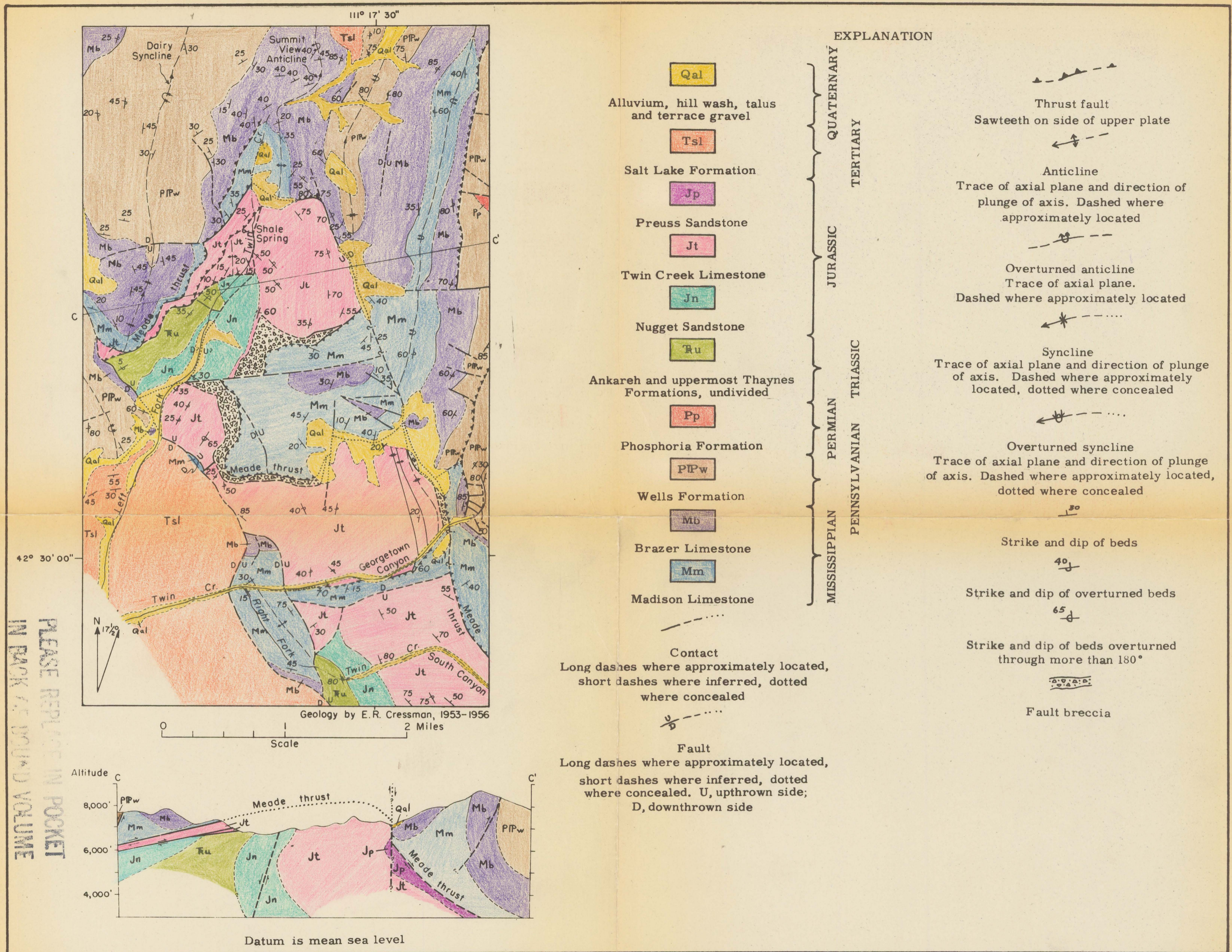
FIGURE 5 GEOLOGIC MAP AND CROSS SECTION OF THE LEFT FORK OF TWIN CREEK AND GEORGETOWN CANYON AREA
