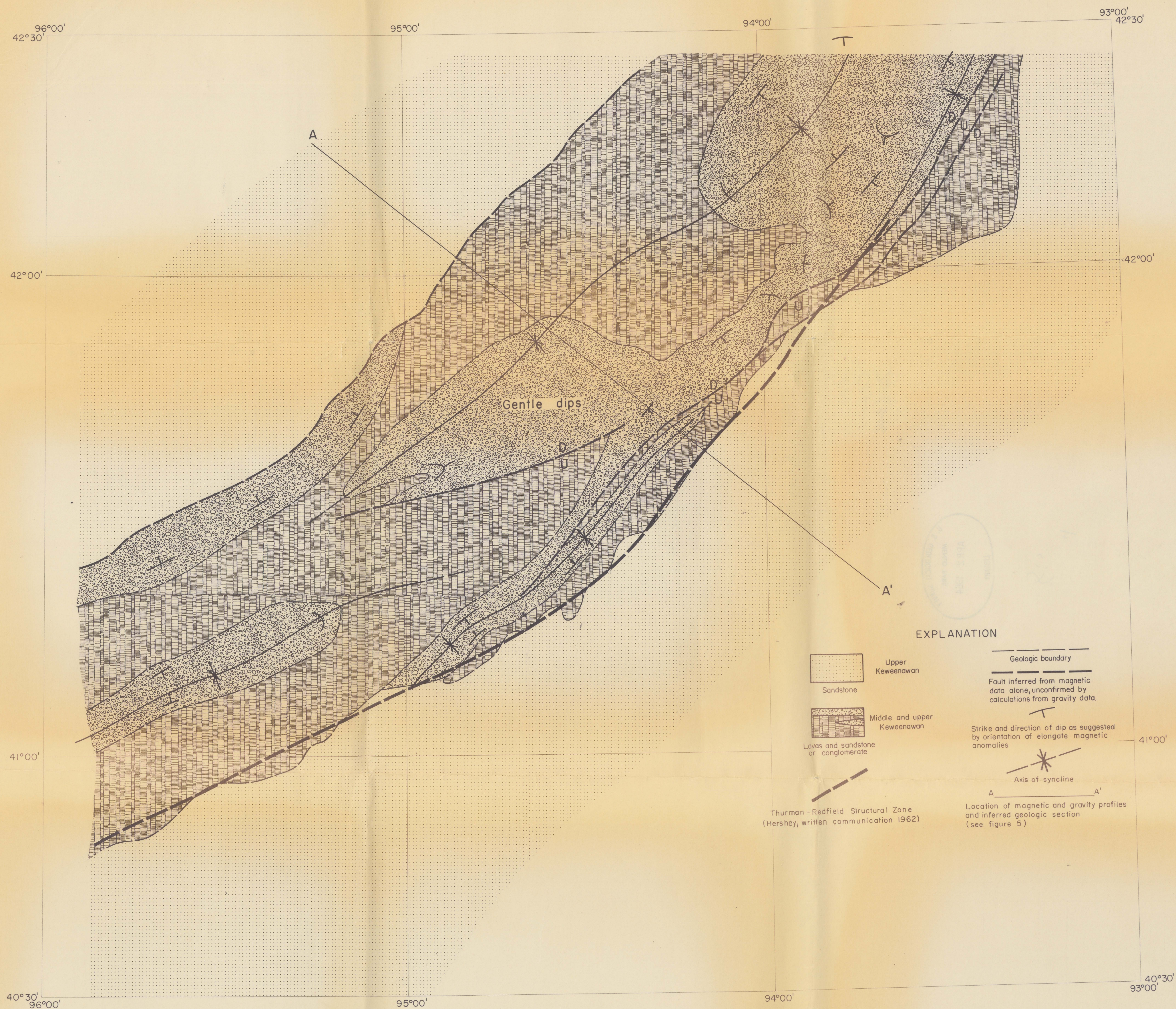
Figure 4 Geologic map of the Precambrian rocks of central and southwestern Iowa as derived from geophysical data
