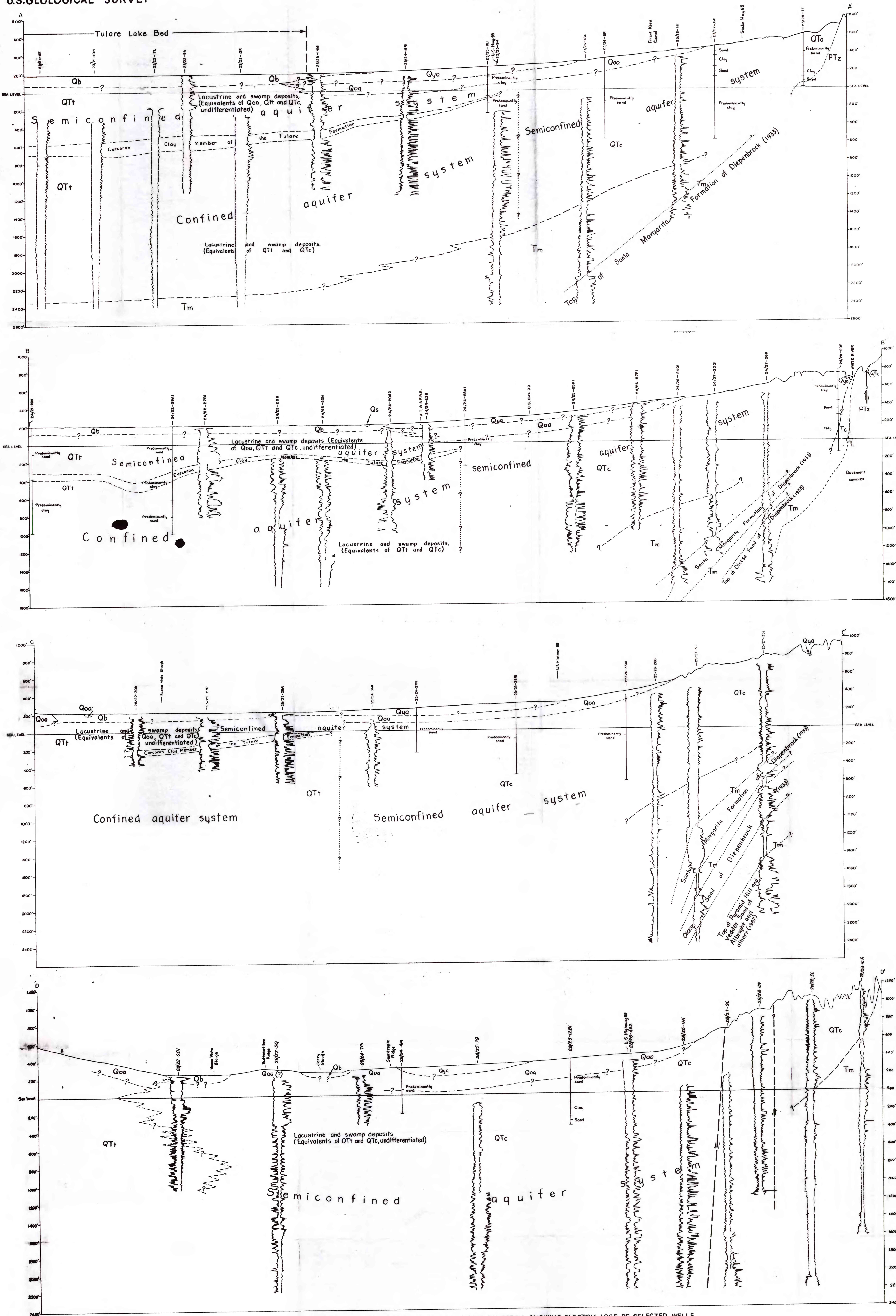
FIGURE 4. — GEOLOGIC SECTIONS, TERRA BELLA-LOST HILLS AREA, CALIFORNIA, SHOWING ELECTRIC LOGS OF SELECTED WELLS Vertical scale 26 times horizontal scale
