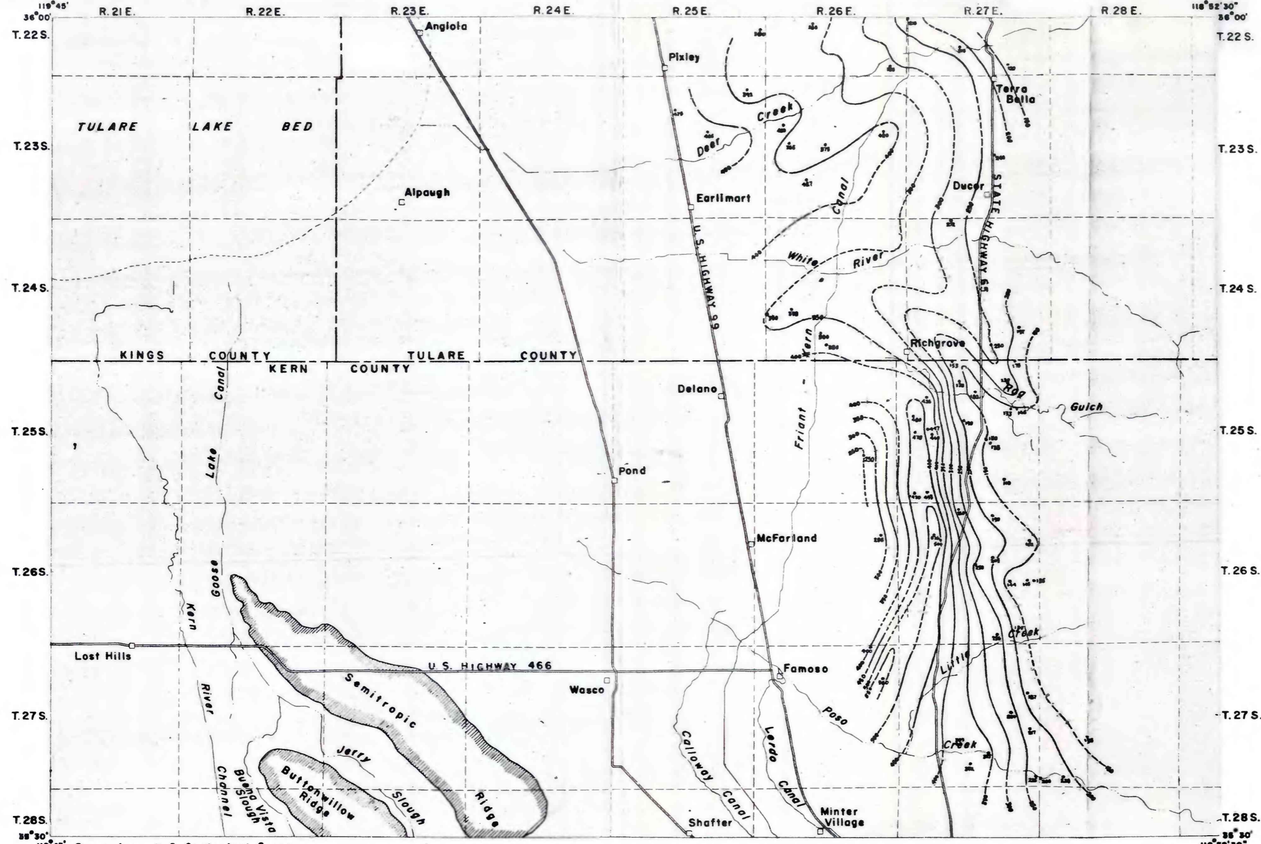
FIGURE 7.-MAP SHOWING LINES OF EQUAL THICKNESS OF THE SANTA MARGARITA FORMATION OF DIEPENBROCK(1933)
