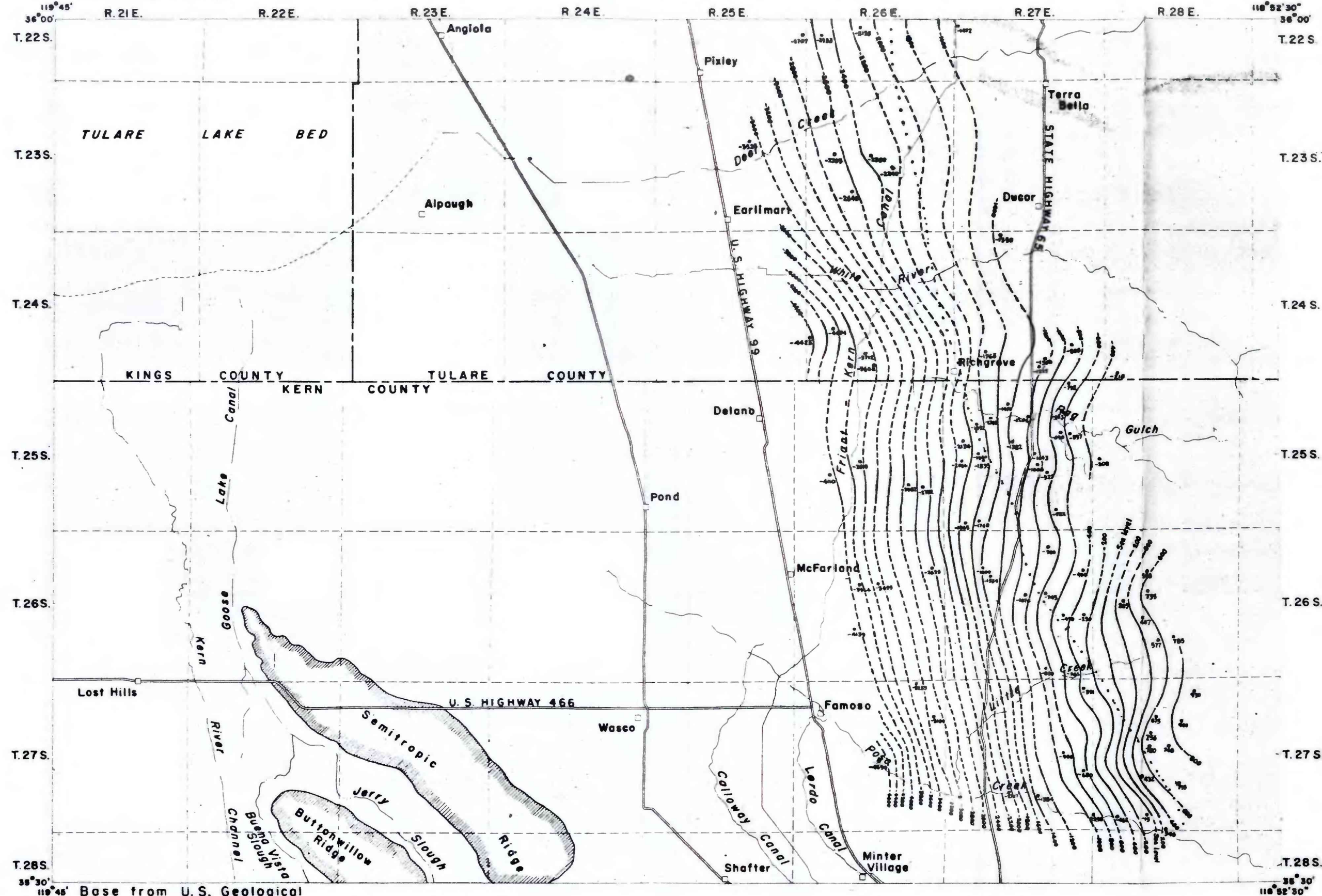
FIGURE 8.-MAP SHOWING SUBSURFACE CONTOURS ON TOP OF THE OLCESE SAND OF DIEPENBROCK(1933)
