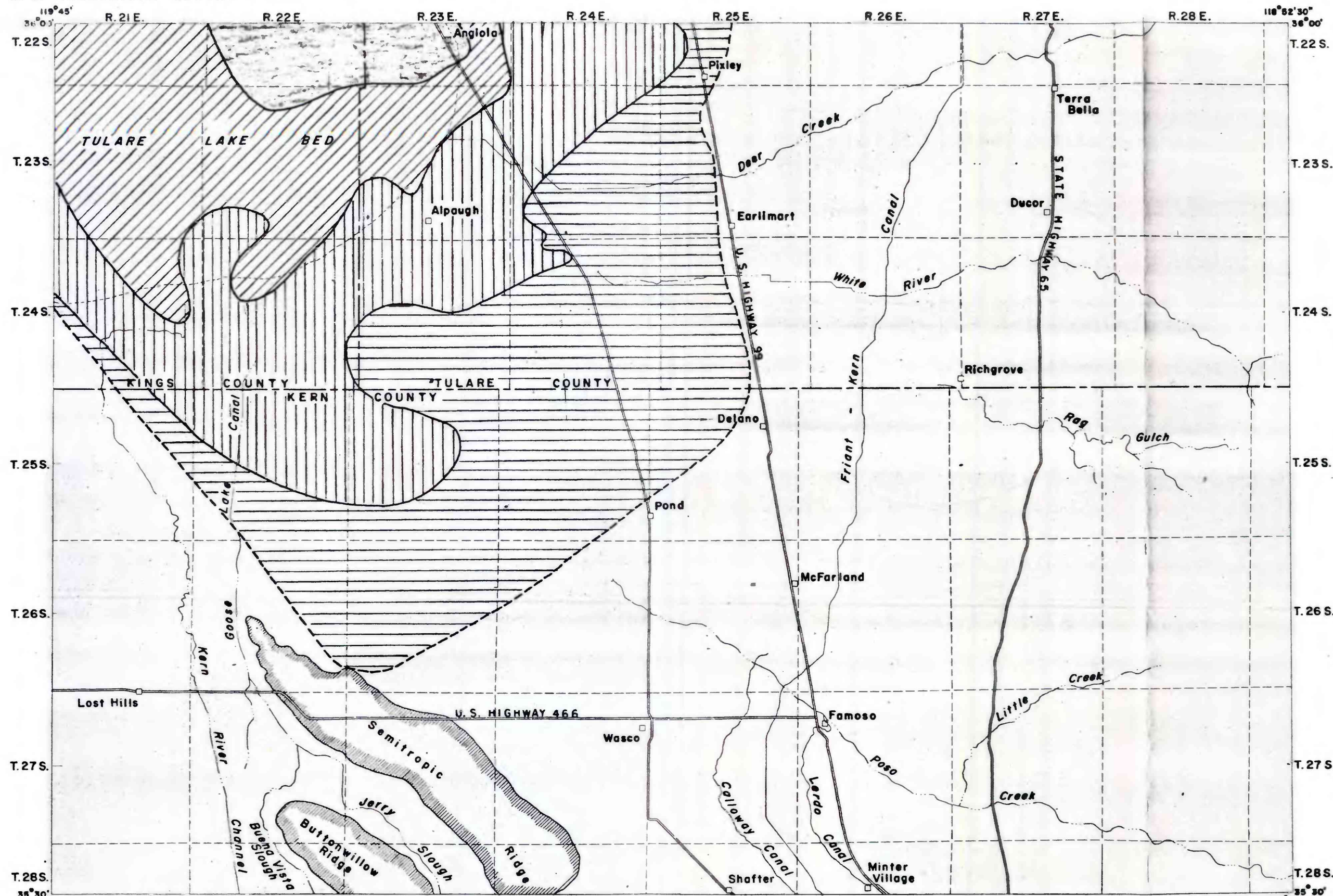
FIGURE 10.- MAP SHOWING EXTENT AND APPROXIMATE THICKNESS OF THE CORCORAN CLAY MEMBER OF THE TULARE FORMATION
