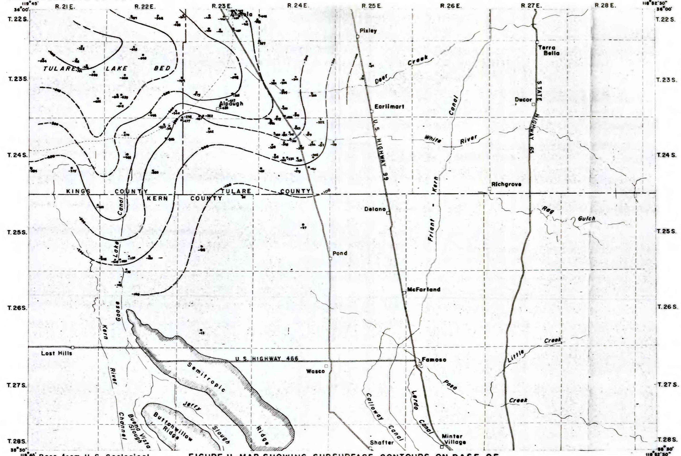
FIGURE II-MAP SHOWING SUBSURFACE CONTOURS ON BASE OF CORCORAN CLAY MEMBER OF TULARE FORMATION
