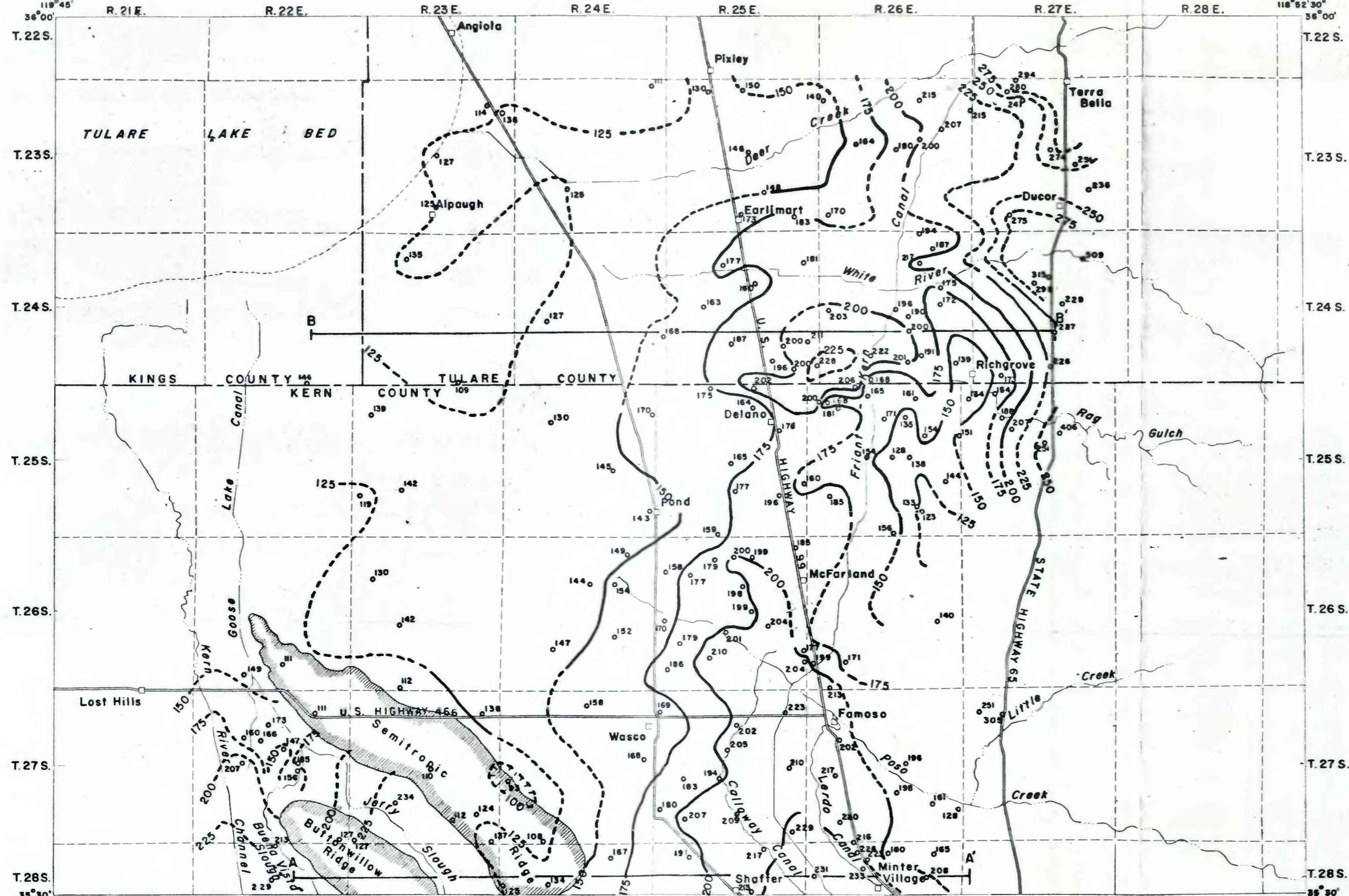
FIGURE 25.-MAP SHOWING WATER-LEVEL CONTOURS OF THE PRINCIPAL PUMPED ZONE, SPRING 1959
