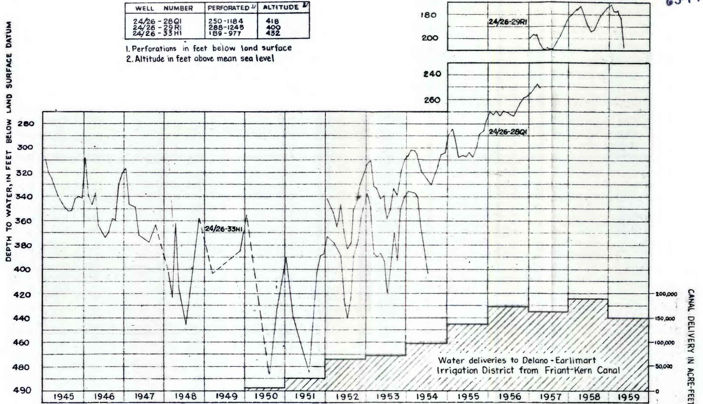
FIGURE 27. - HYDROGRAPHS OF WELLS 24/26-28QI, 29 RI, AND 33HI AND WATER DELIVERIES TO DELANO-EARLIMART IRRIGATION DISTRICT FROM FRIANT-KERN CANAL
