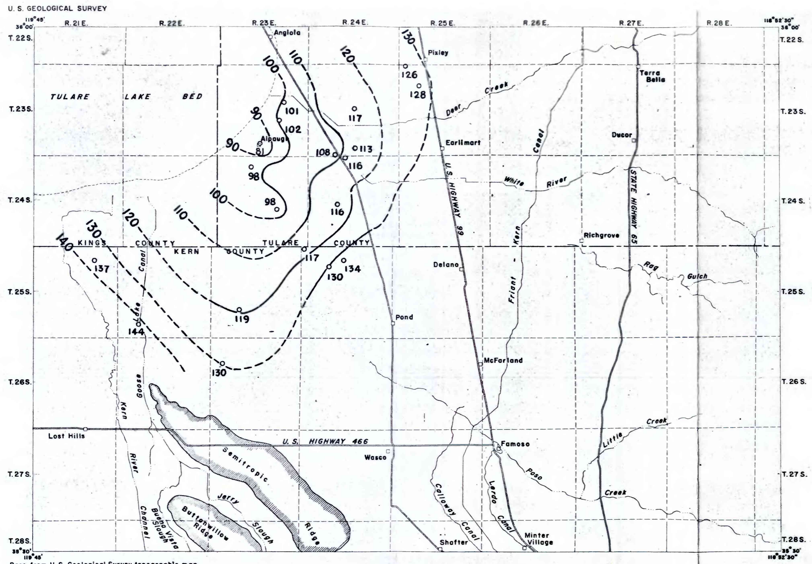
FIGURE 30.- MAP SHOWING CONTOURS OF THE PIEZOMETRIC SURFACE OF THE CONFINED AQUIFER SYSTEM, SPRING 1959
