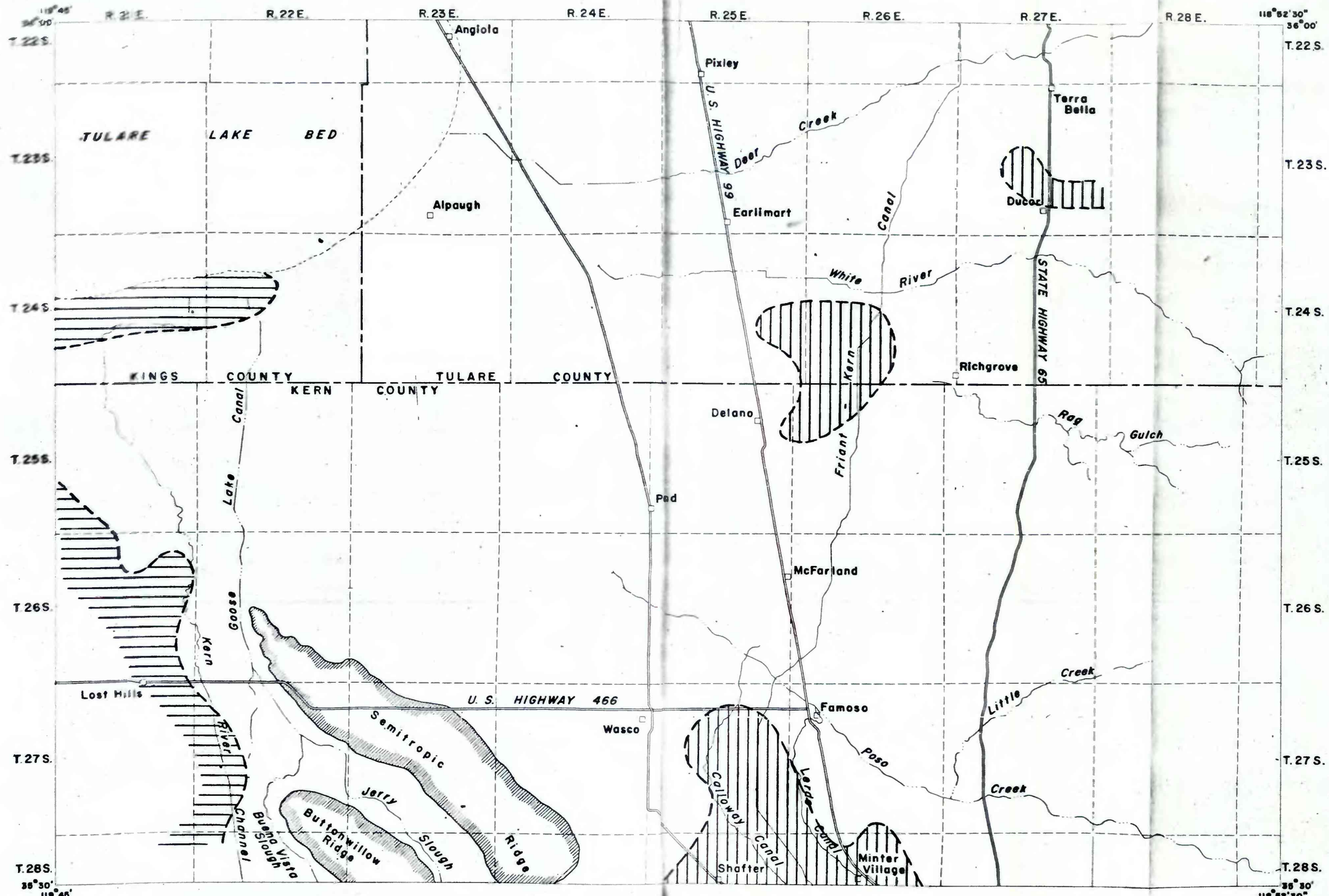
FIGURE 39.- MAP SHOWING HIGH BORON AND NITRATE CONCENTRATIONS IN THE TERRA BELLA-LOST HILLS AREA, CALIFORNIA
