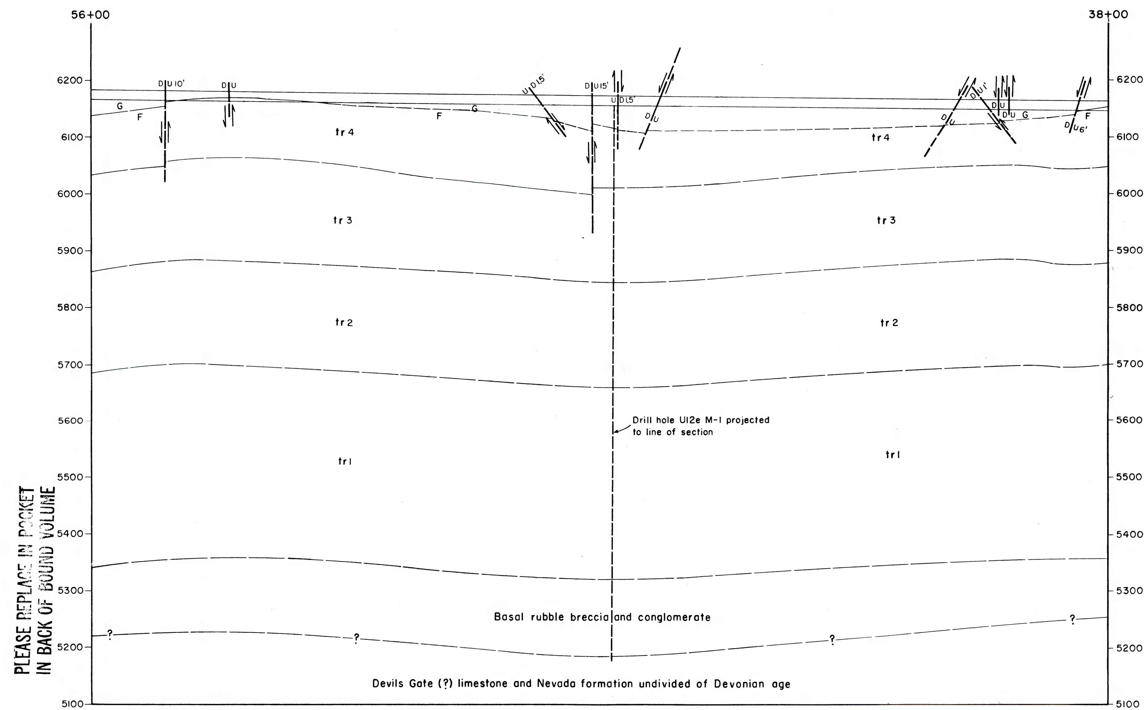
FIGURE 2-CROSS SECTIONS OF THE RIGHT WALL OF THE UI2e TUNNEL, NEVADA TEST SITE, NYE COUNTY, NEVADA
