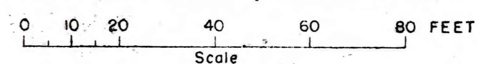
FIGURE 6- GEOLOGIC MAP OF THE U12e.03 TUNNEL, NEVADA TEST SITE, NYE COUNTY, NEVADA
