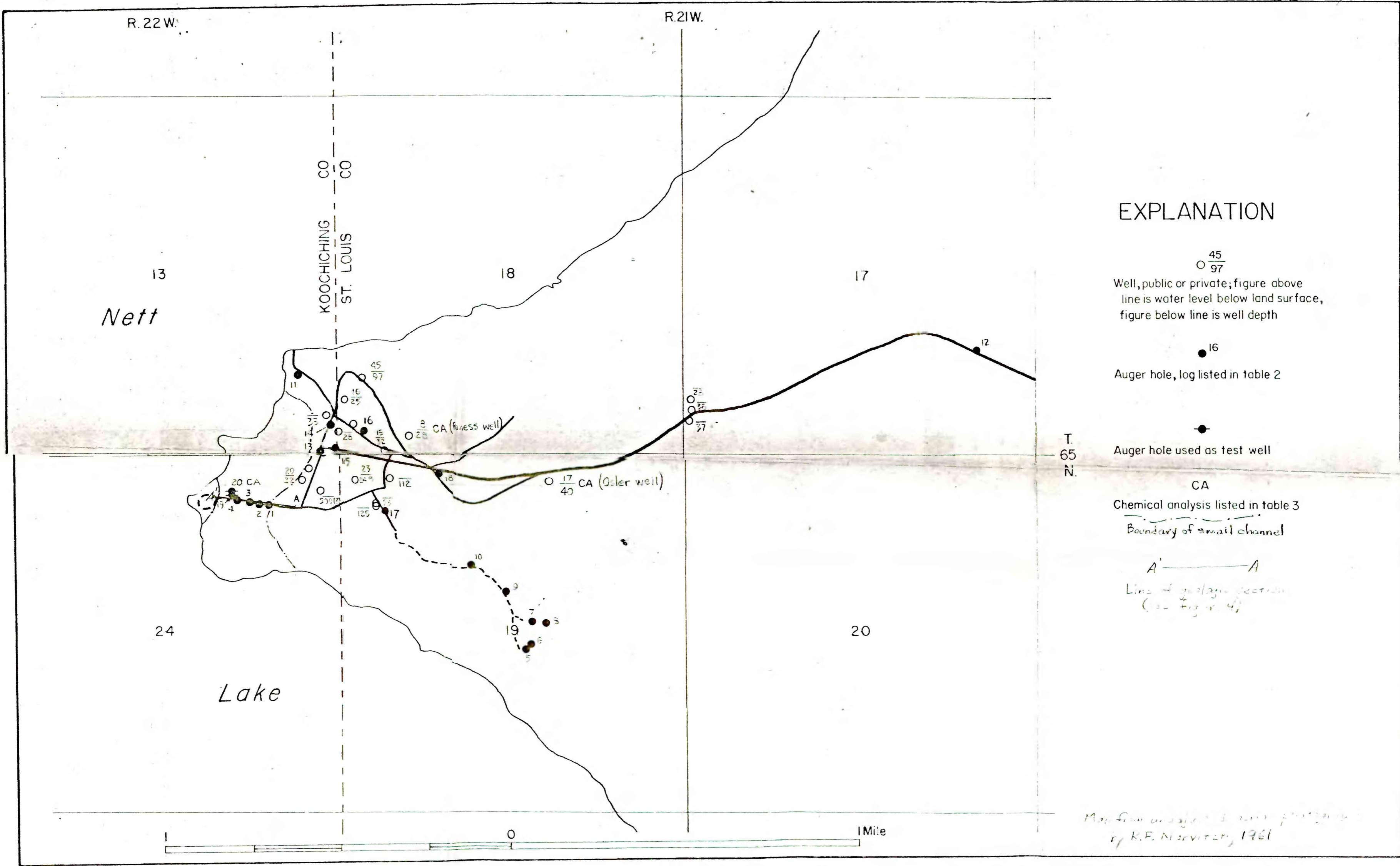
Figure 3. — Locations of wells and auger holes in the vicinity of the Village of Nett Lake, Minnesota
