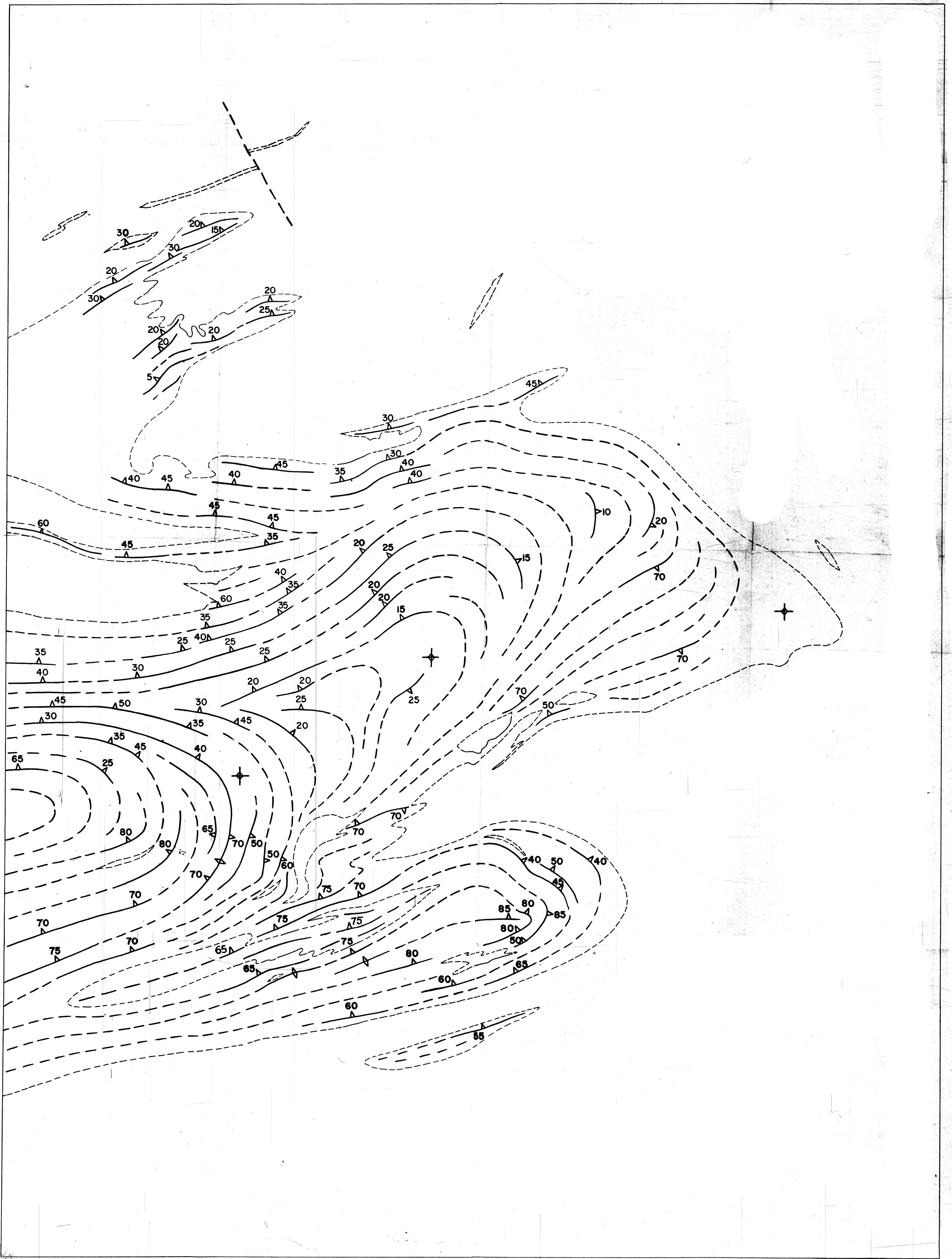
Form lines, Potter Hill Granite Gneiss
