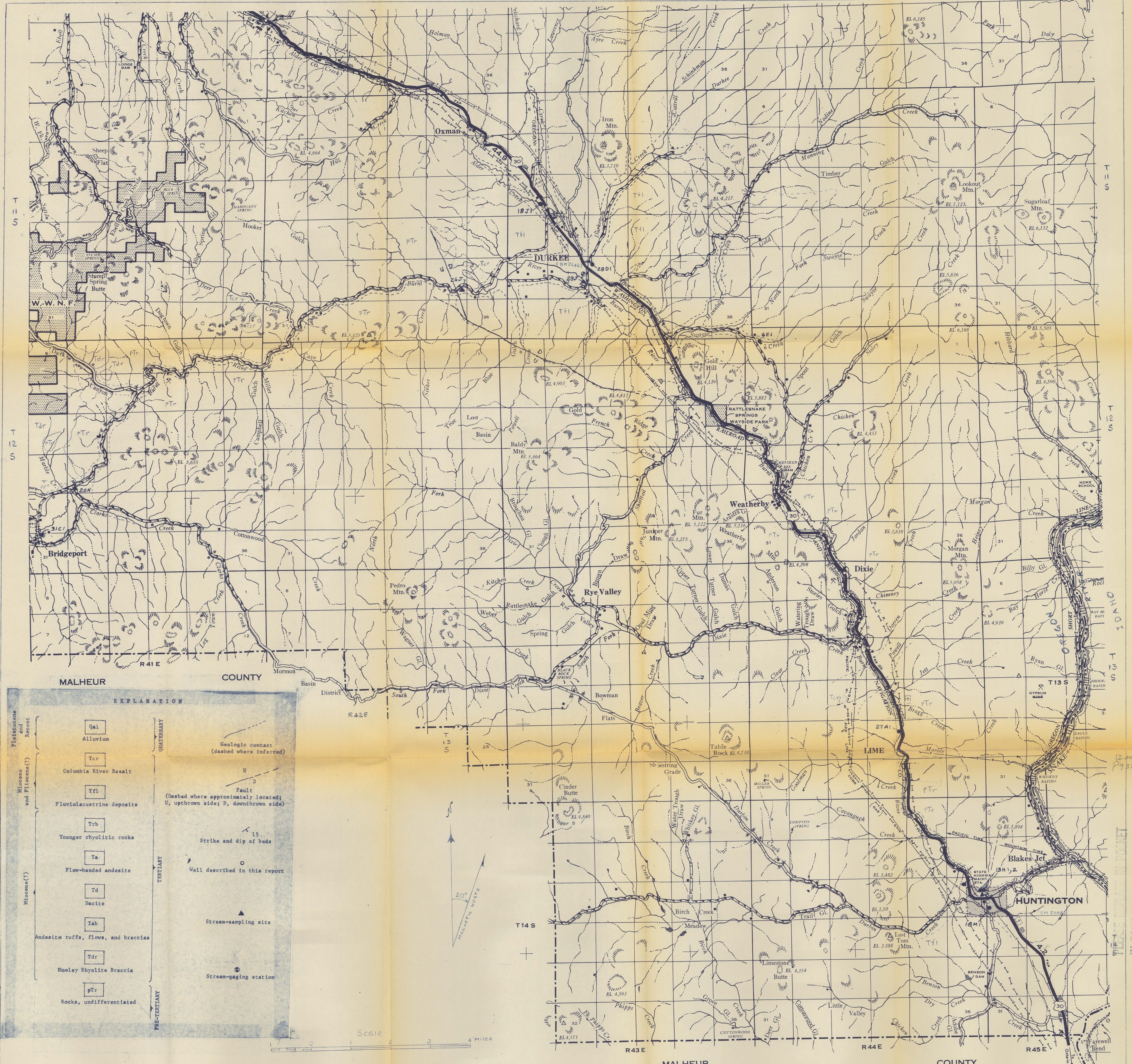
Figure 2A.--Map of eastern part of Burnt River Valley area showing distribution of rock units and locations of wells, stream-gaging stations and stream-sampling points.
