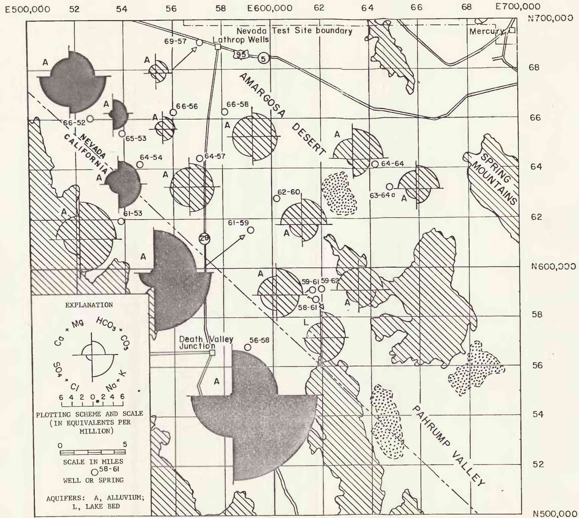
Figure 6.--MAP OF THE SOUTHWESTERN PART OF THE AMARGOSA DESERT SHOWING CHEMISTRY OF GROUND WATER. SODIUM-POTASSIUM TYPE, BLACK; MIXED TYPE, RULED.
