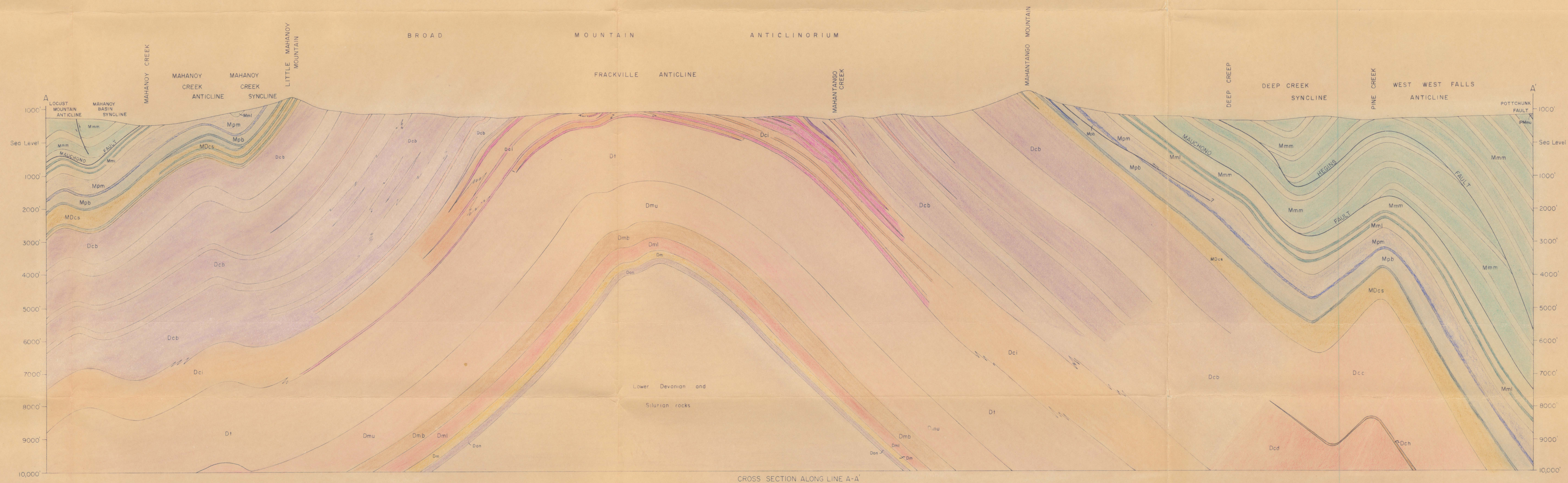
CROSS SECTION ALONG LINE A-A'
