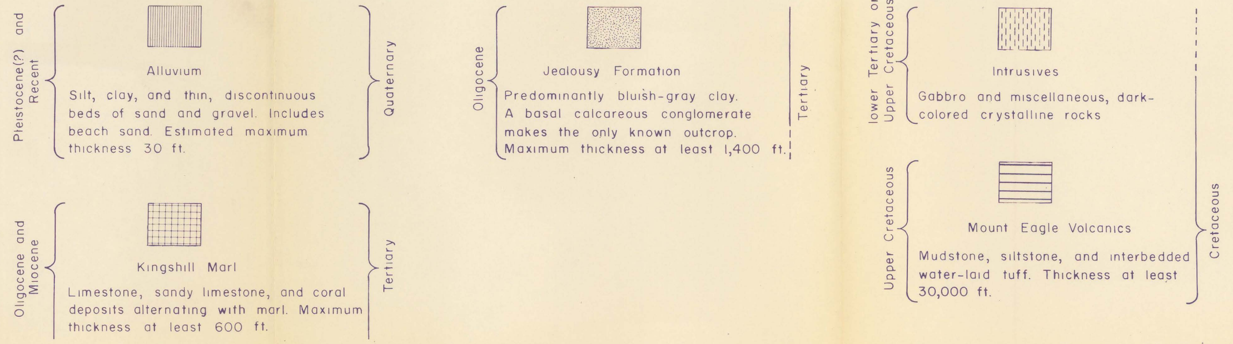
Figure 3.--Generalized geologic map of St. Croix.
