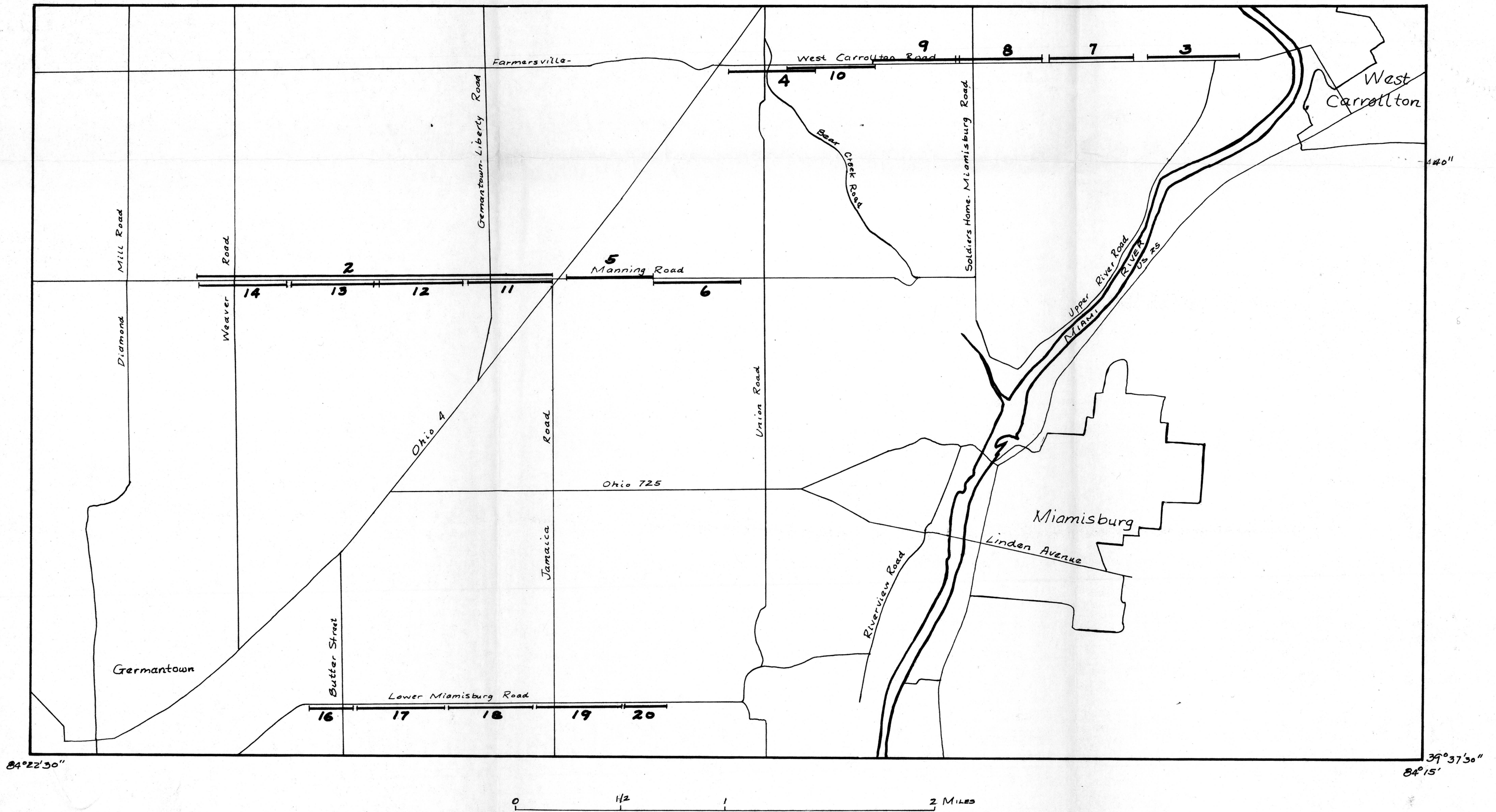
FIGURE 1 - Seismic lines shot in Miamisburg quadrangle, Ohio in 1963
