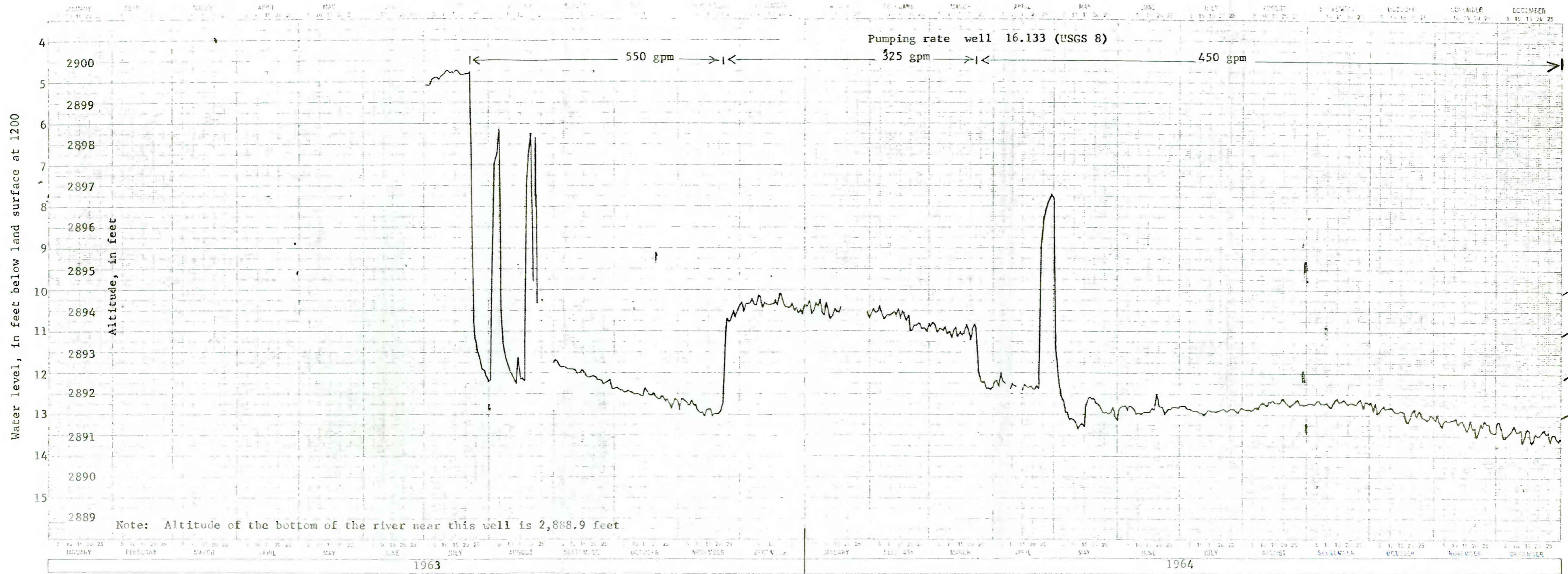
Figure 6.--Graph showing fluctuation of water level in well 17.444 (USGS 11)
