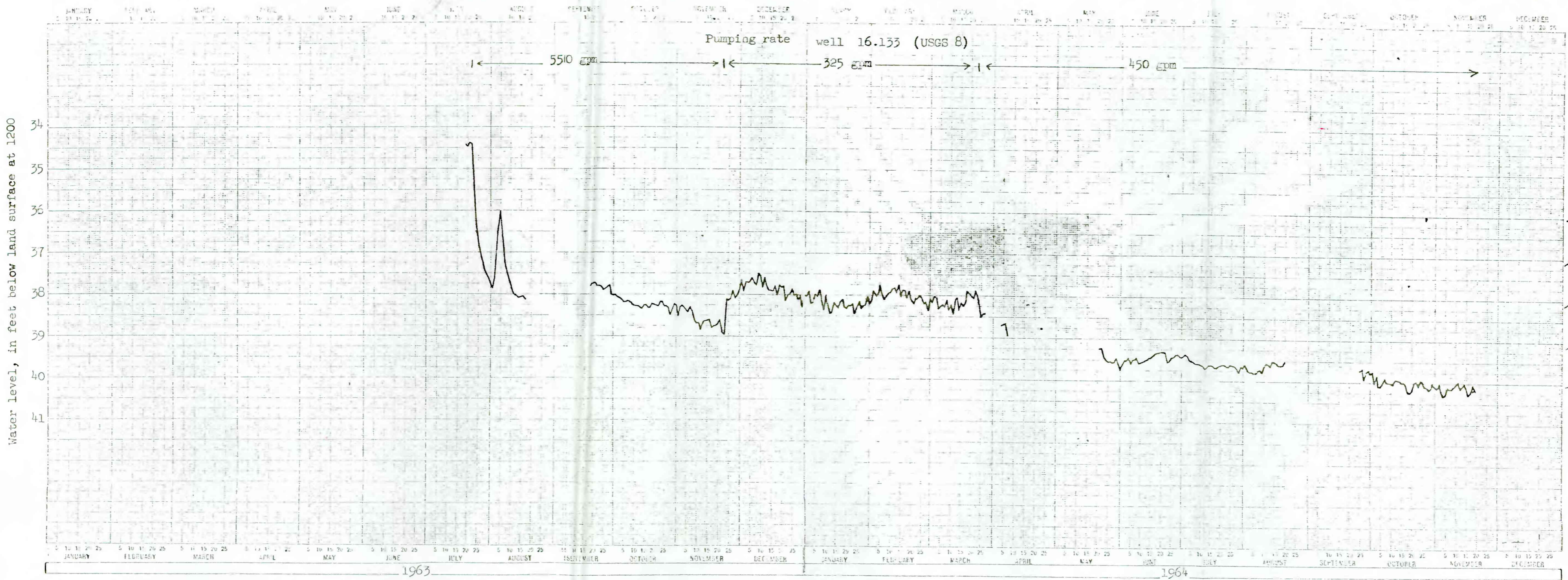
Figure 10.--Graph showing fluctuation of water level in well 8.111 (USGS 3)
