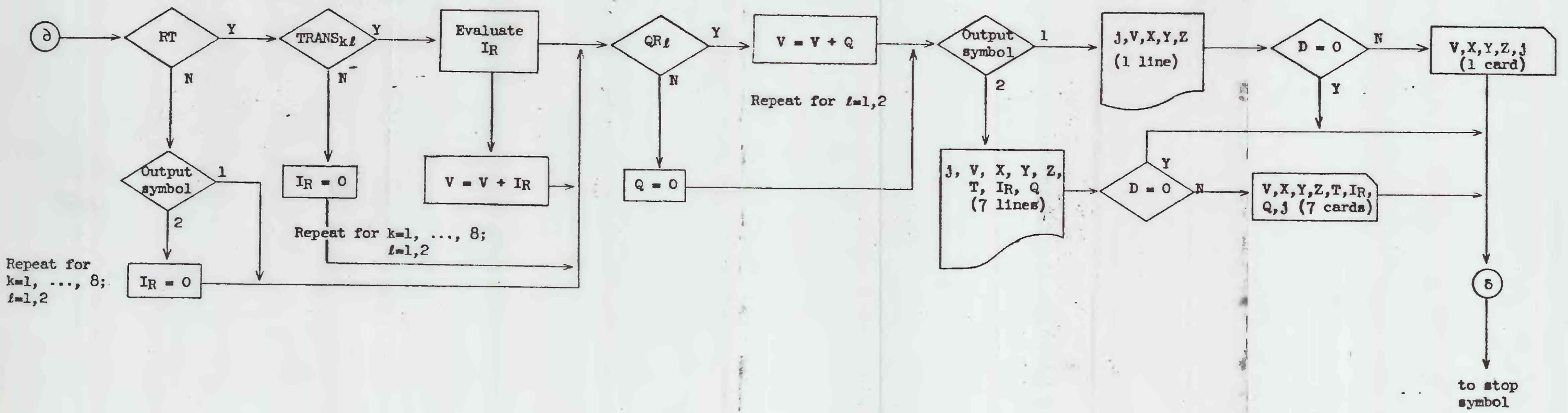
Figure 7. Flow diagram of computation and output section of the program. See figure 4. See appendix B for explanation of symbols.
