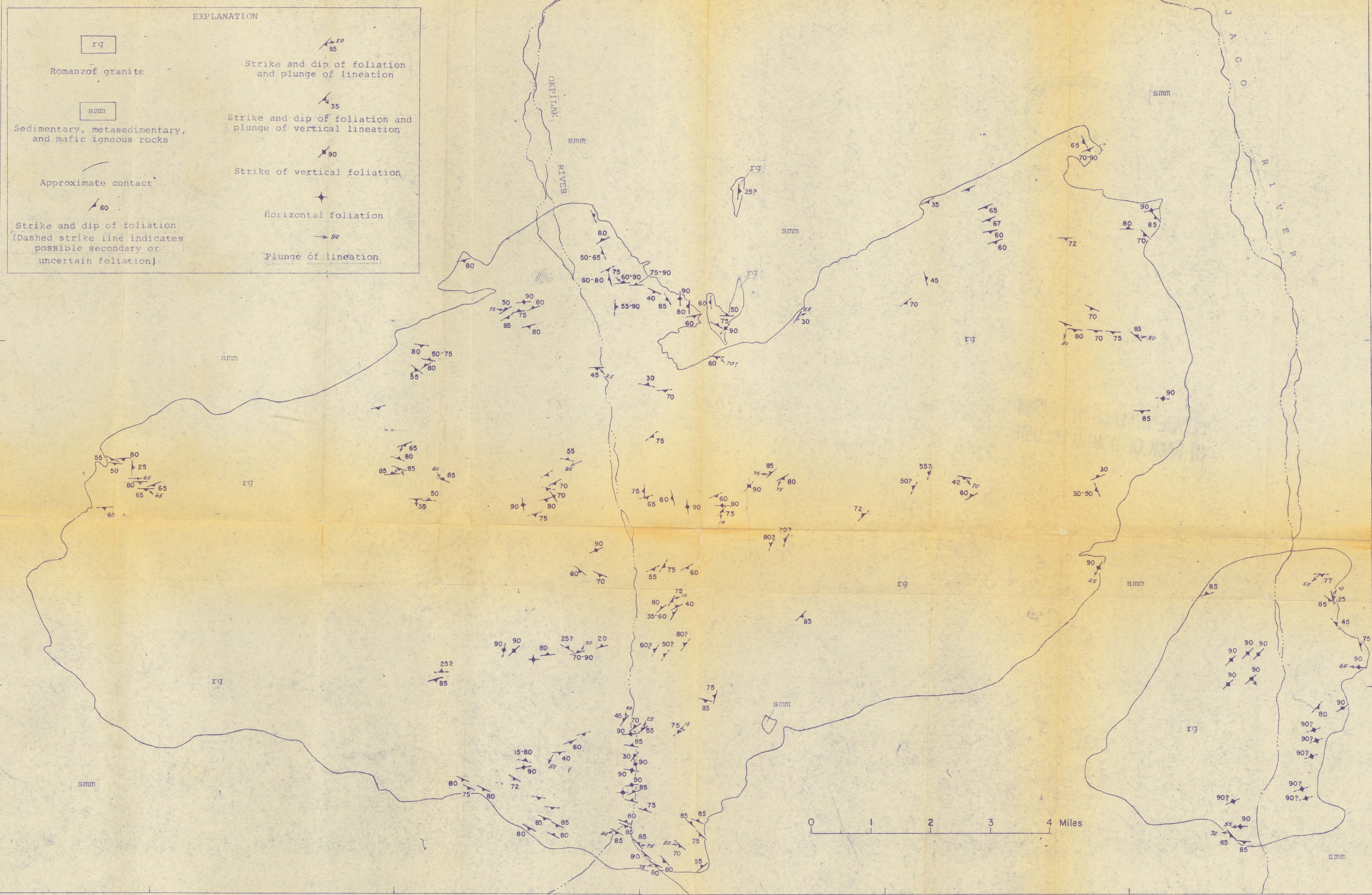
PLATE 6. MAP SHOWING FELDSPAR FOLIATION AND LINEATION IN ROMANZOF GRANITE, ROMANZOF MOUNTAINS, ALASKA.
