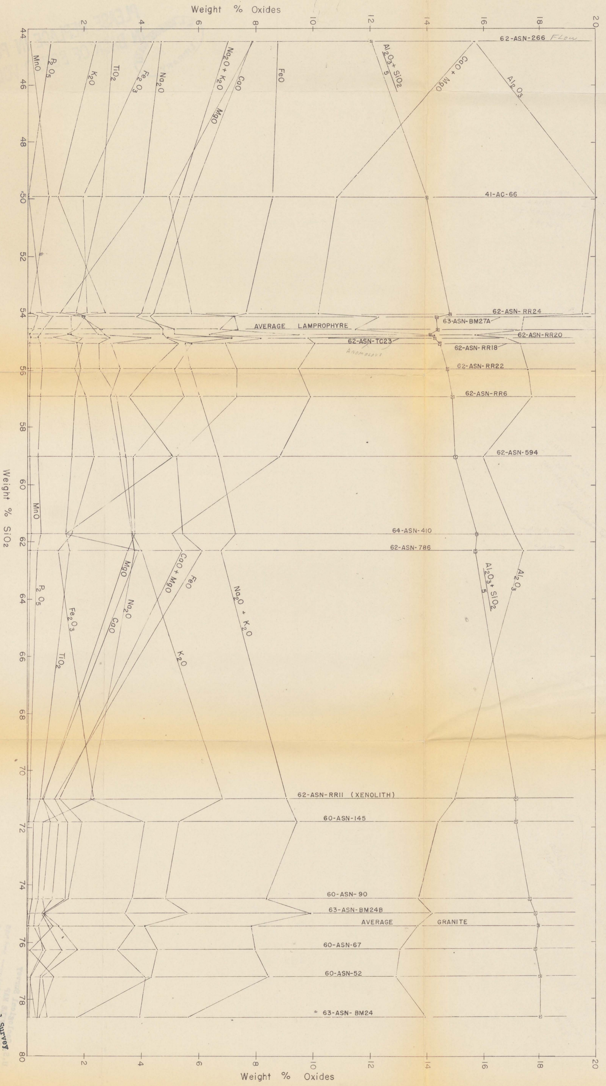
FIGURE 22 LARSEN DIAGRAM SHOWING VARIATION IN OXIDES IN IGNEOUS ROCKS OF THE YORK MOUNTAINS, SEWARD PENINSULA, ALASKA
