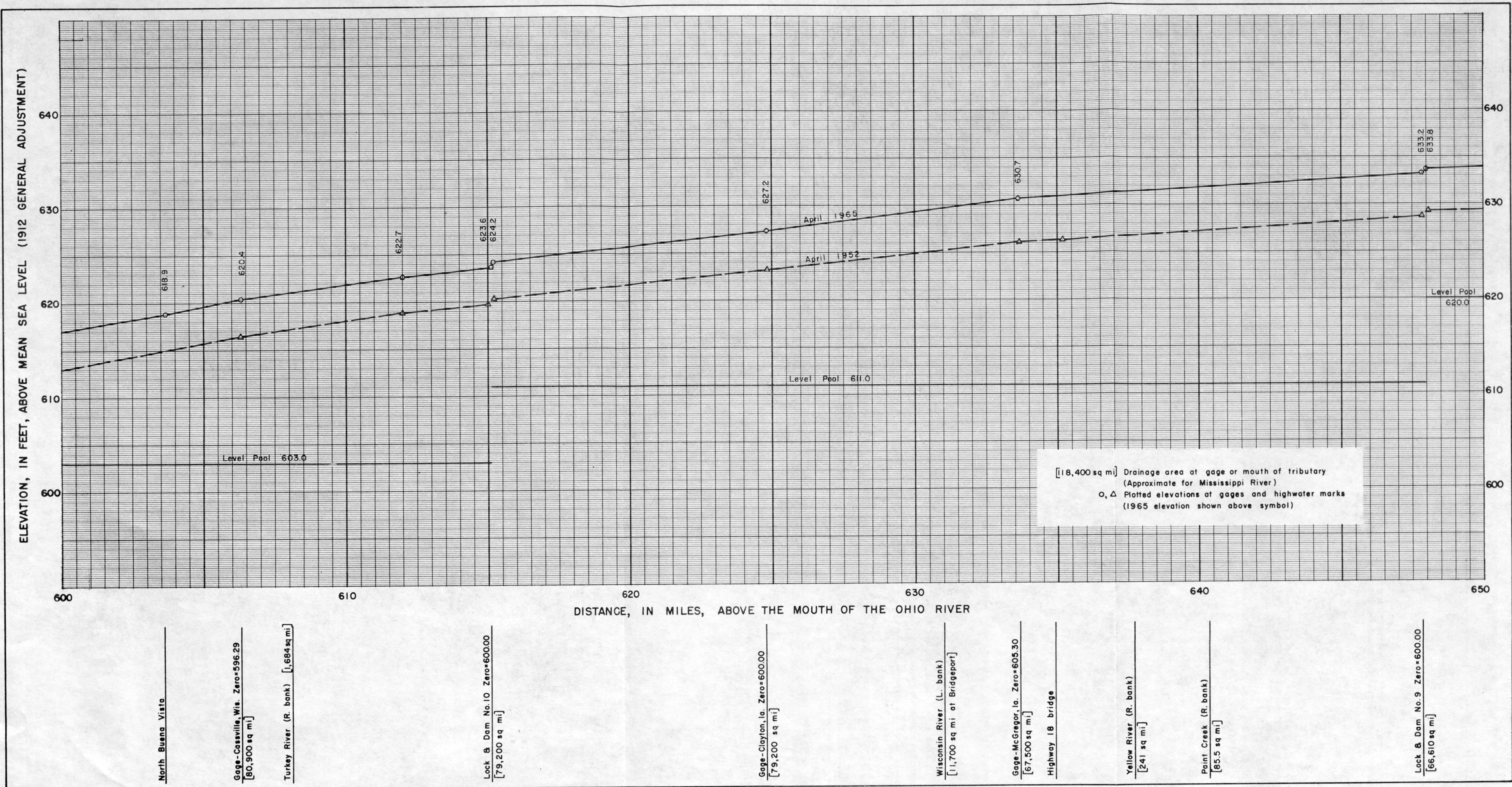
Plate 7. Selected profiles of the Mississippi River floods, mile 600 to mile 650.
