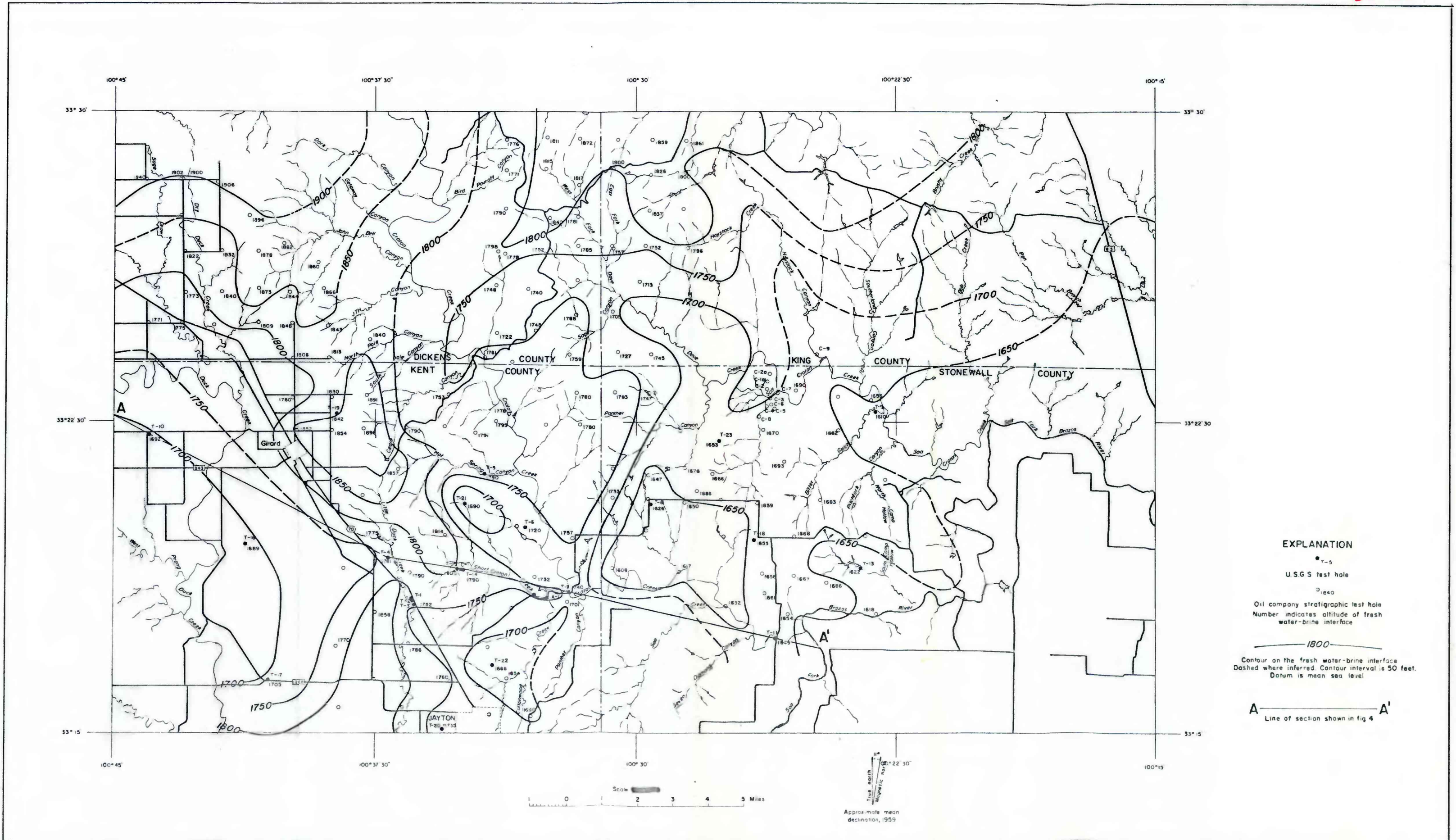
Figure 3.-Map of the Croton Creek-Salt Croton Creek area showing the location of test holes and contours on the fresh water-brine interface
