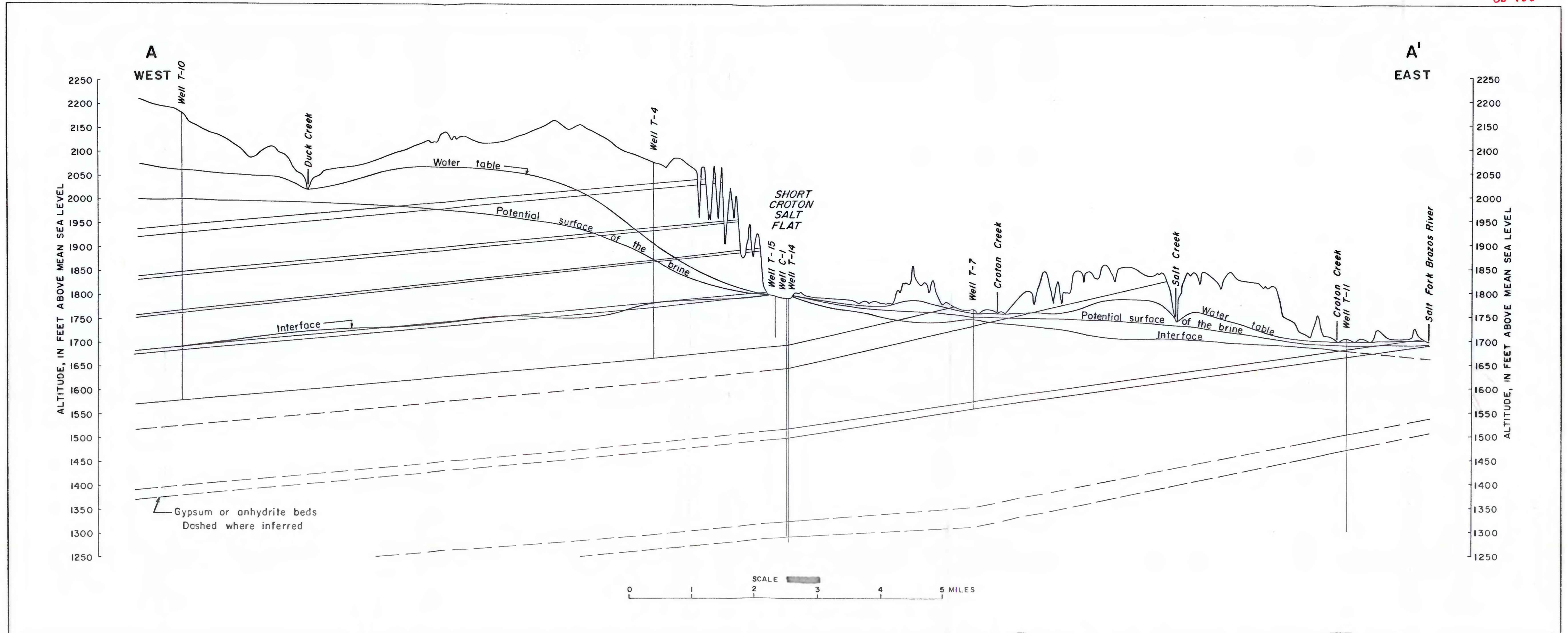
Figure 4.-East-west section through the Croton Creek-Salt Croton Creek area showing geologic and hydrologic relations
