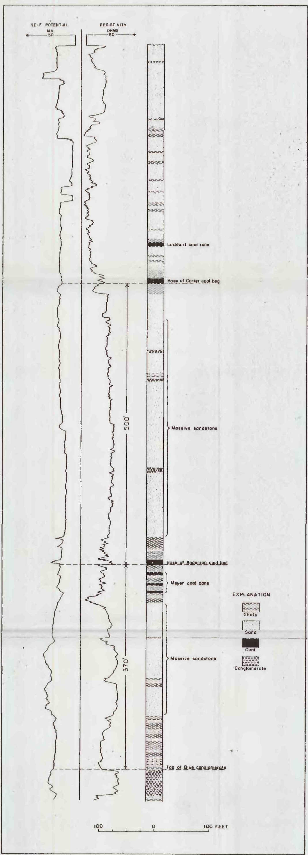
FIGURE 1—Composite stratigraphic section, upper portion of Tye Formation in the Eden Ridge coal field. Data furnished by Pacific Power and Light Co.
