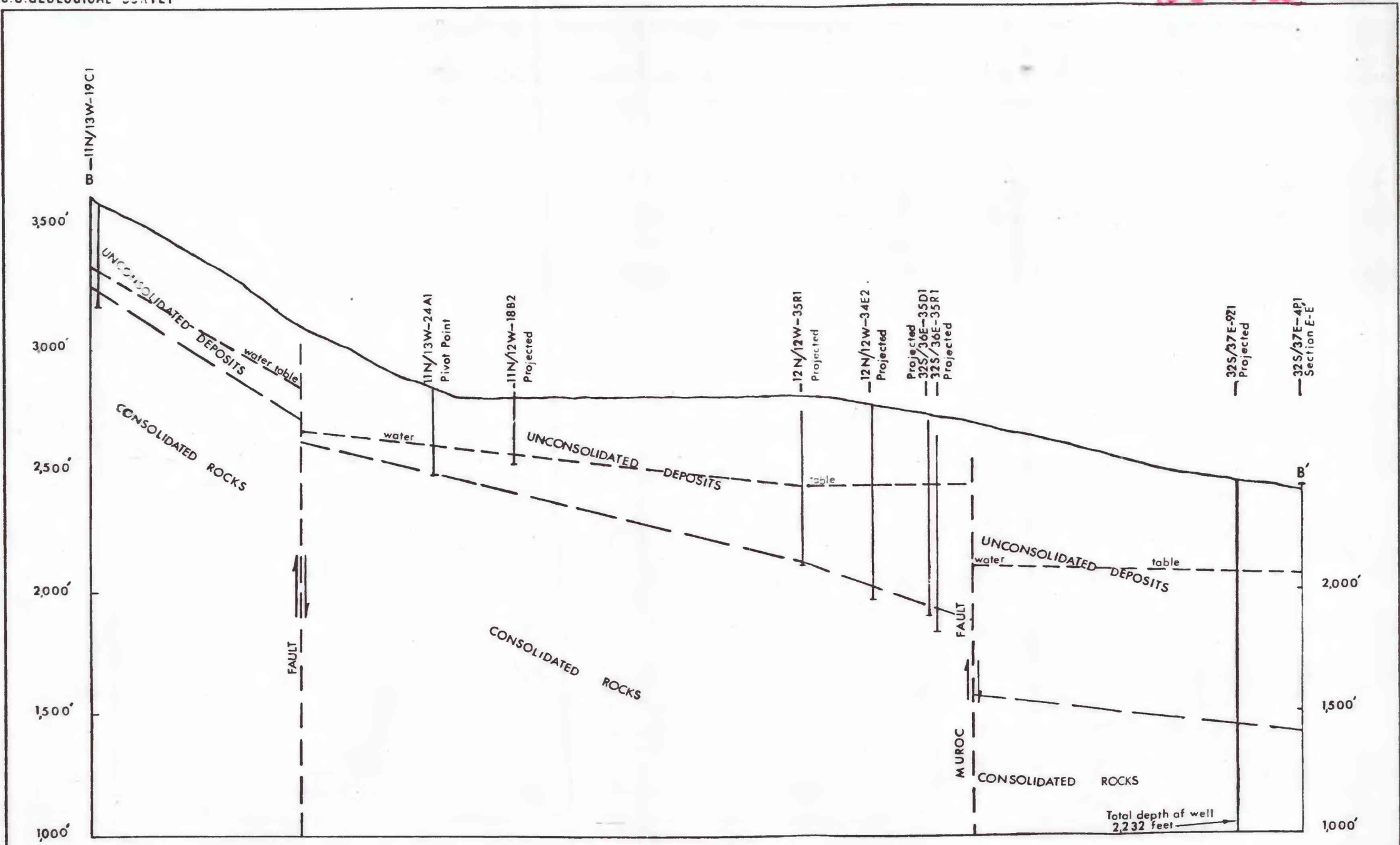
GEOLOGIC SECTION B-B' IN FREMONT VALLEY SHOWING WATER-LEVEL PROFILE
